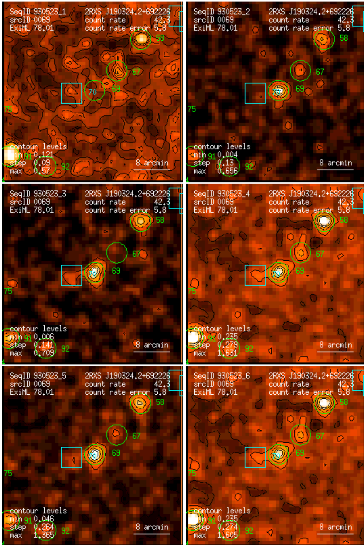
Figure 69: RASS 930523: detection 0069: band rate images, Gaussian filter: (1) PSPC channels 11 – 41, (2) 52 – 90, (3) 91 – 201, (4) 11 – 235, (5) 52 – 201, (6) 11 – 201. Broad band rates in counts/ks. Band rate contour levels in counts/ks/arcmin 2 .
