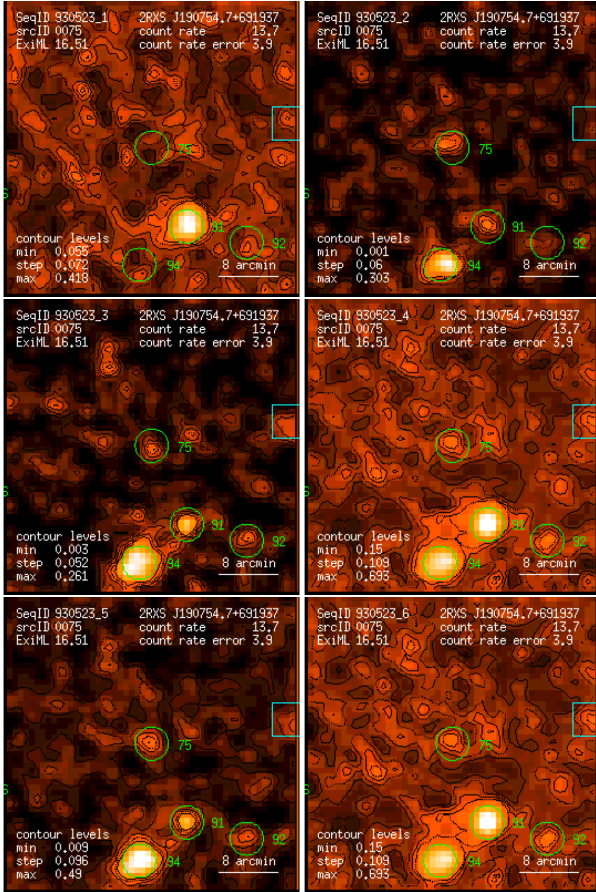
Figure 75: RASS 930523: detection 0075: band rate images, Gaussian filter: (1) PSPC channels 11 – 41, (2) 52 – 90, (3) 91 – 201, (4) 11 – 235, (5) 52 – 201, (6) 11 – 201. Broad band rates in counts/ks. Band rate contour levels in counts/ks/arcmin 2 .
