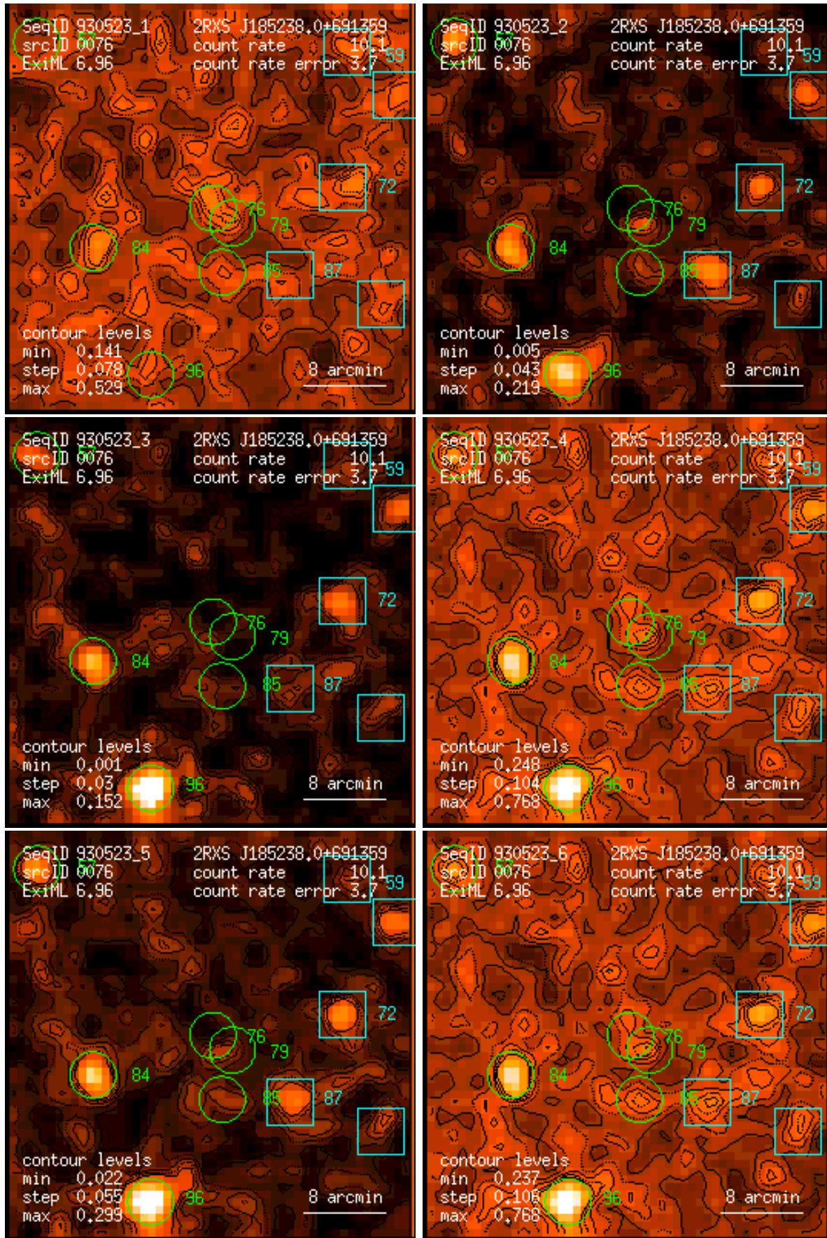
Figure 76: RASS 930523: detection 0076: band rate images, Gaussian filter: (1) PSPC channels 11 – 41, (2) 52 – 90, (3) 91 – 201, (4) 11 – 235, (5) 52 – 201, (6) 11 – 201. Broad band rates in counts/ks. Band rate contour levels in counts/ks/arcmin 2 .
