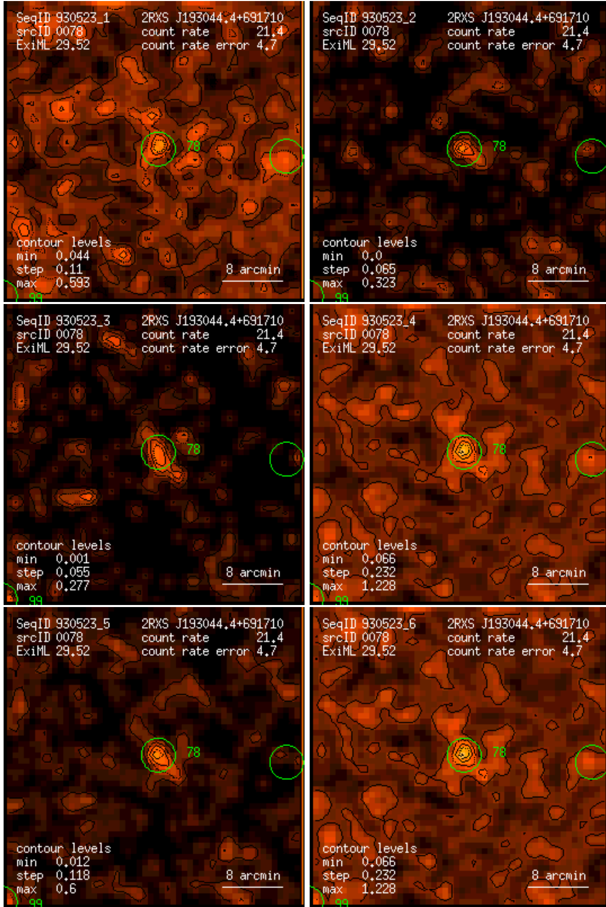
Figure 78: RASS 930523: detection 0078: band rate images, Gaussian filter: (1) PSPC channels 11 – 41, (2) 52 – 90, (3) 91 – 201, (4) 11 – 235, (5) 52 – 201, (6) 11 – 201. Broad band rates in counts/ks. Band rate contour levels in counts/ks/arcmin 2 .
