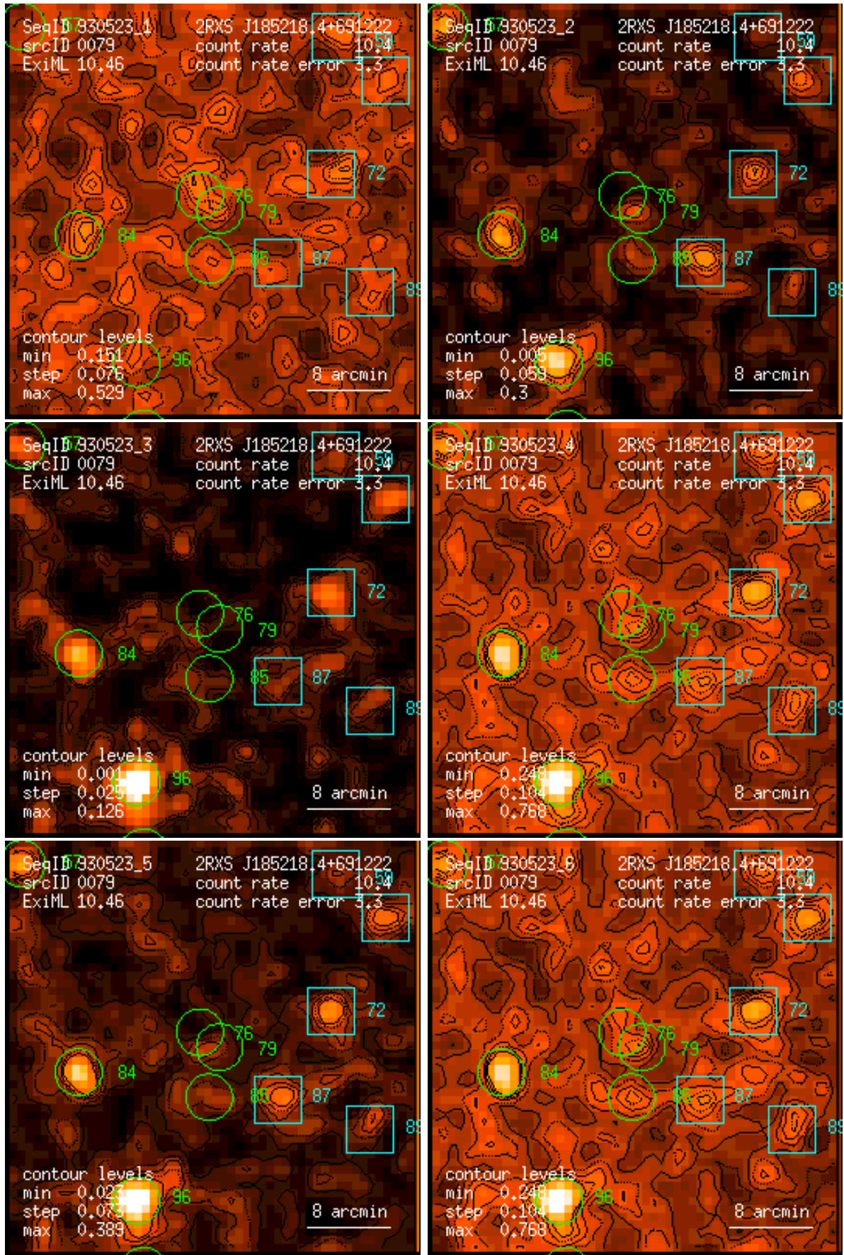
Figure 79: RASS 930523: detection 0079: band rate images, Gaussian filter: (1) PSPC channels 11 – 41, (2) 52 – 90, (3) 91 – 201, (4) 11 – 235, (5) 52 – 201, (6) 11 – 201. Broad band rates in counts/ks. Band rate contour levels in counts/ks/arcmin 2 .
