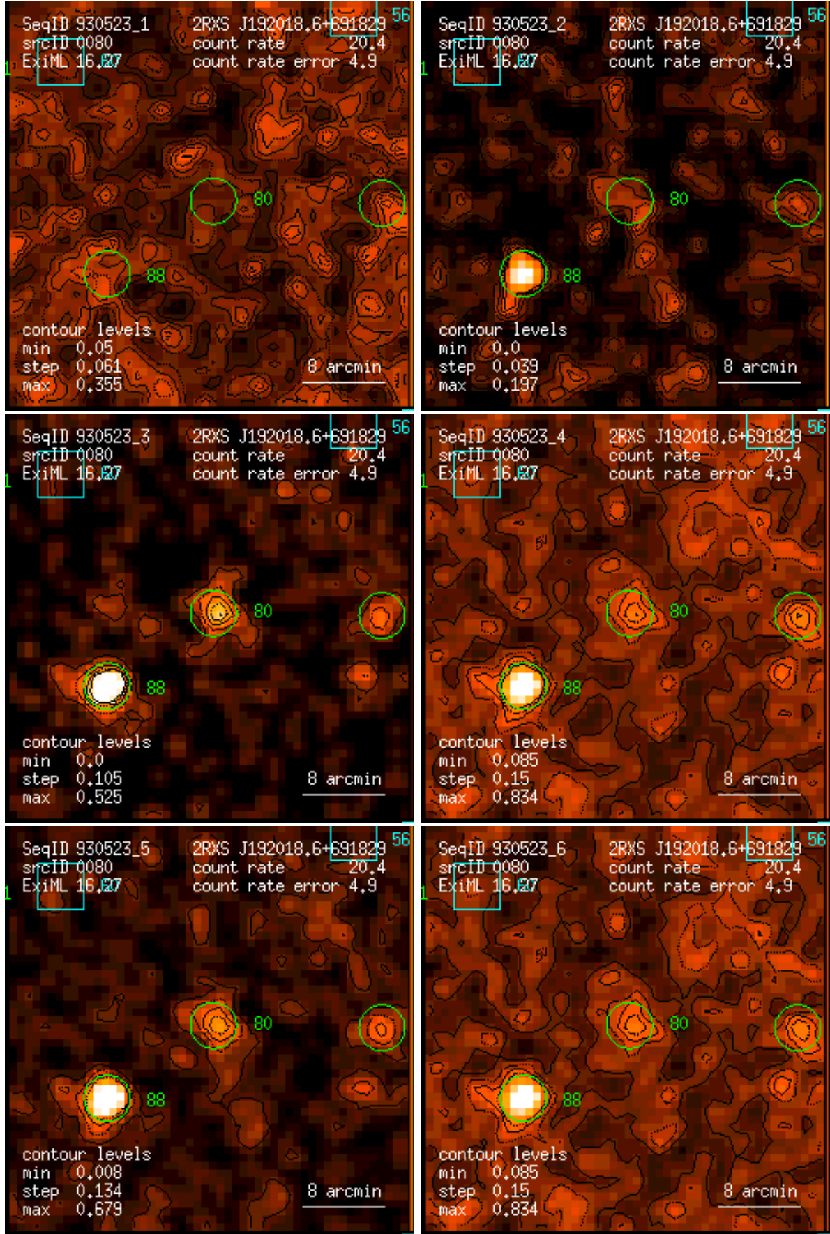
Figure 80: RASS 930523: detection 0080: band rate images, Gaussian filter: (1) PSPC channels 11 – 41, (2) 52 – 90, (3) 91 – 201, (4) 11 – 235, (5) 52 – 201, (6) 11 – 201. Broad band rates in counts/ks. Band rate contour levels in counts/ks/arcmin 2 .
