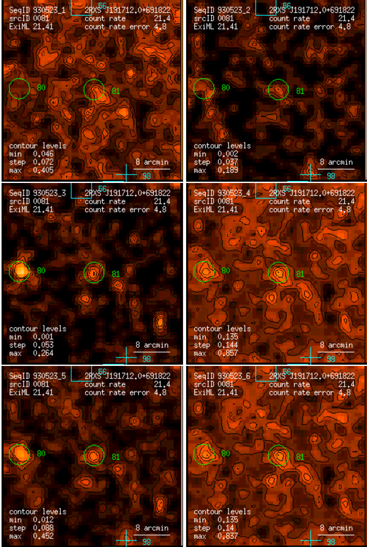
Figure 81: RASS 930523: detection 0081: band rate images, Gaussian filter: (1) PSPC channels 11 – 41, (2) 52 – 90, (3) 91 – 201, (4) 11 – 235, (5) 52 – 201, (6) 11 – 201. Broad band rates in counts/ks. Band rate contour levels in counts/ks/arcmin 2 .
