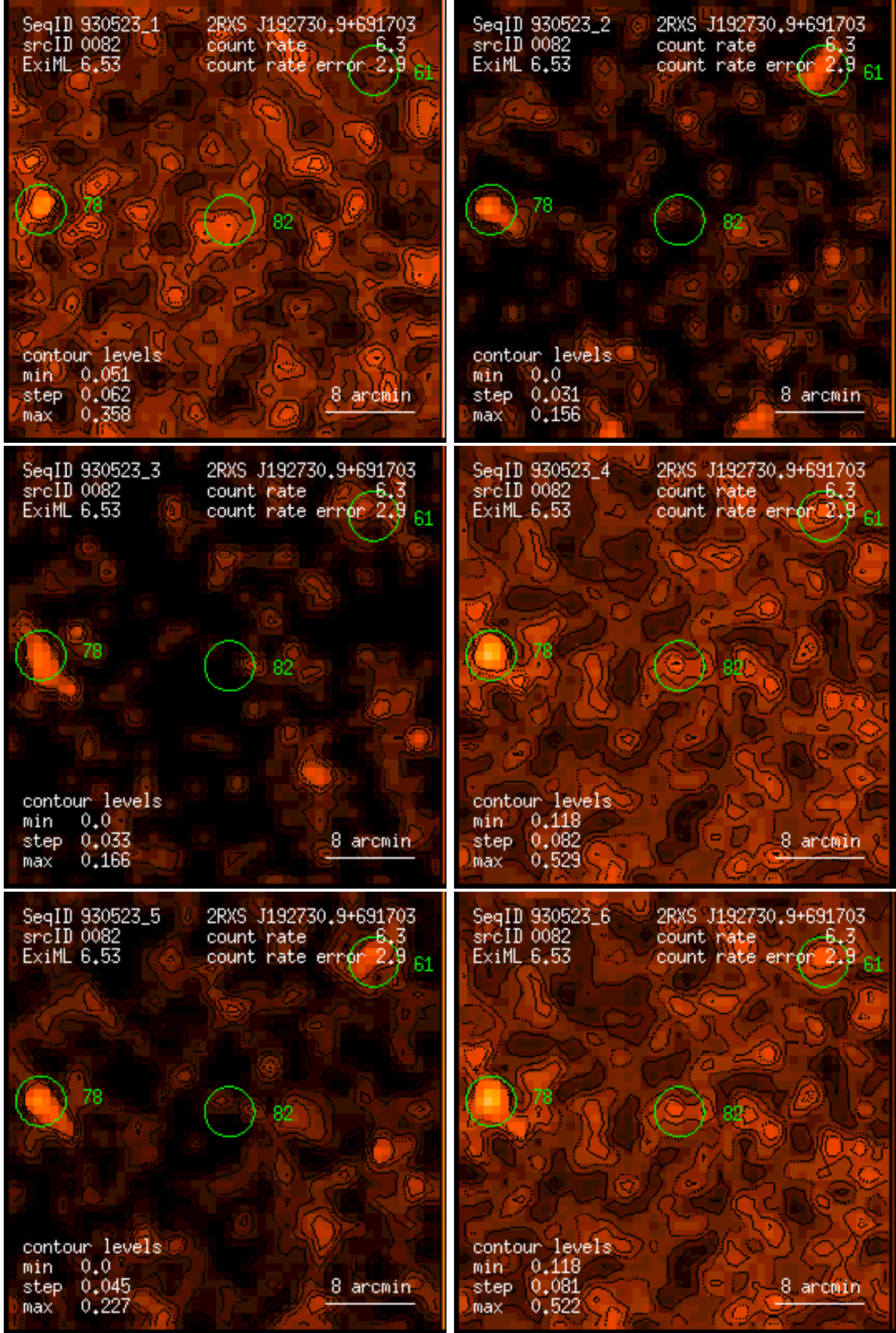
Figure 82: RASS 930523: detection 0082: band rate images, Gaussian filter: (1) PSPC channels 11 – 41, (2) 52 – 90, (3) 91 – 201, (4) 11 – 235, (5) 52 – 201, (6) 11 – 201. Broad band rates in counts/ks. Band rate contour levels in counts/ks/arcmin 2 .
