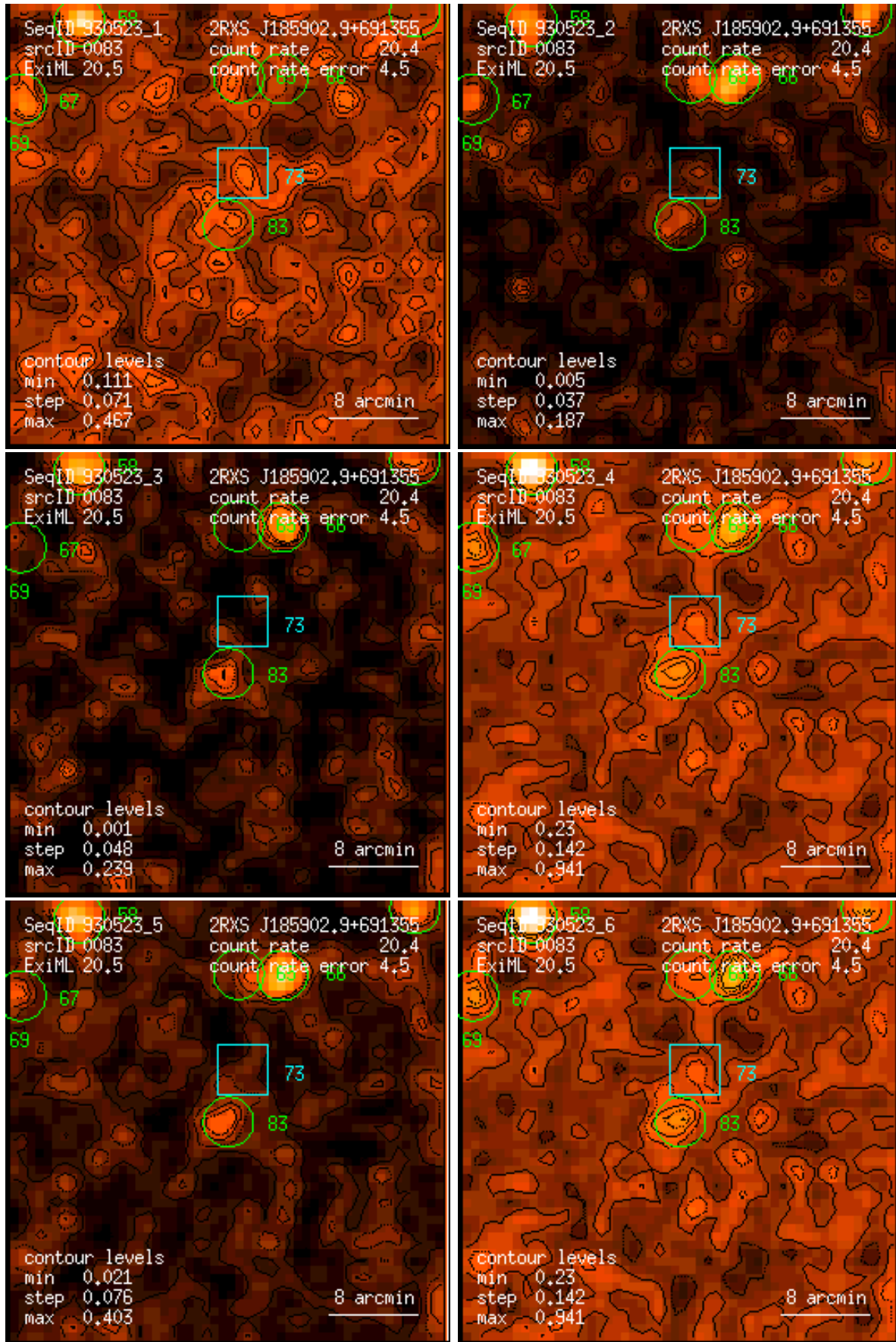
Figure 83: RASS 930523: detection 0083: band rate images, Gaussian filter: (1) PSPC channels 11 – 41, (2) 52 – 90, (3) 91 – 201, (4) 11 – 235, (5) 52 – 201, (6) 11 – 201. Broad band rates in counts/ks. Band rate contour levels in counts/ks/arcmin 2 .
