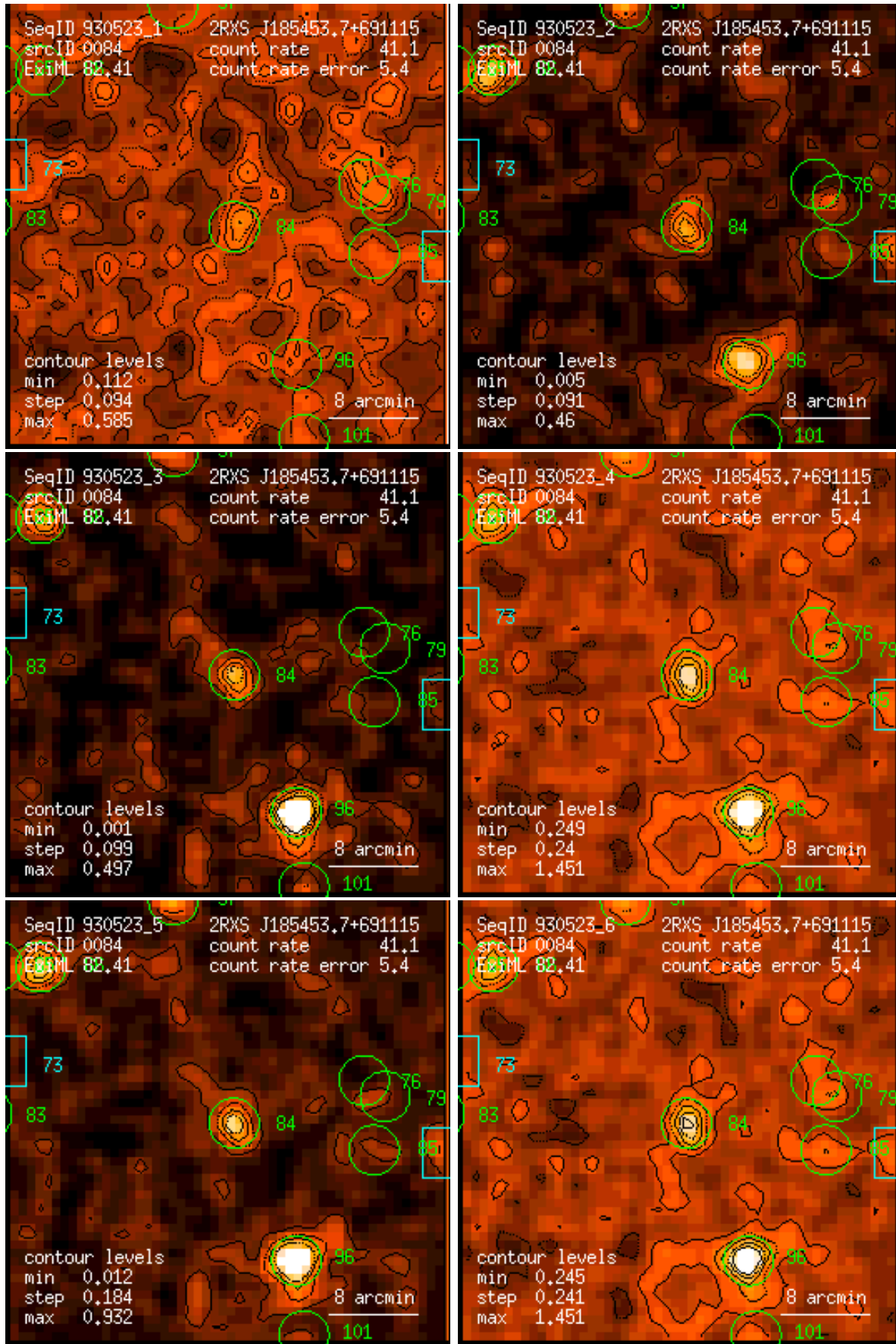
Figure 84: RASS 930523: detection 0084: band rate images, Gaussian filter: (1) PSPC channels 11 – 41, (2) 52 – 90, (3) 91 – 201, (4) 11 – 235, (5) 52 – 201, (6) 11 – 201. Broad band rates in counts/ks. Band rate contour levels in counts/ks/arcmin 2 .
