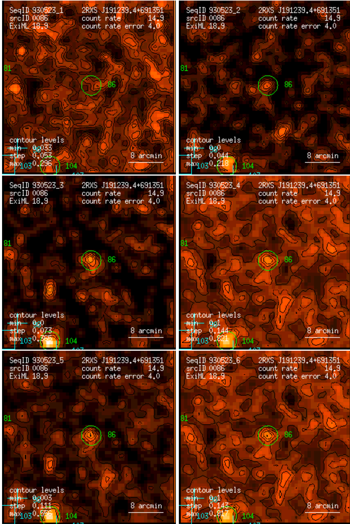
Figure 86: RASS 930523: detection 0086: band rate images, Gaussian filter: (1) PSPC channels 11 – 41, (2) 52 – 90, (3) 91 – 201, (4) 11 – 235, (5) 52 – 201, (6) 11 – 201. Broad band rates in counts/ks. Band rate contour levels in counts/ks/arcmin 2 .
