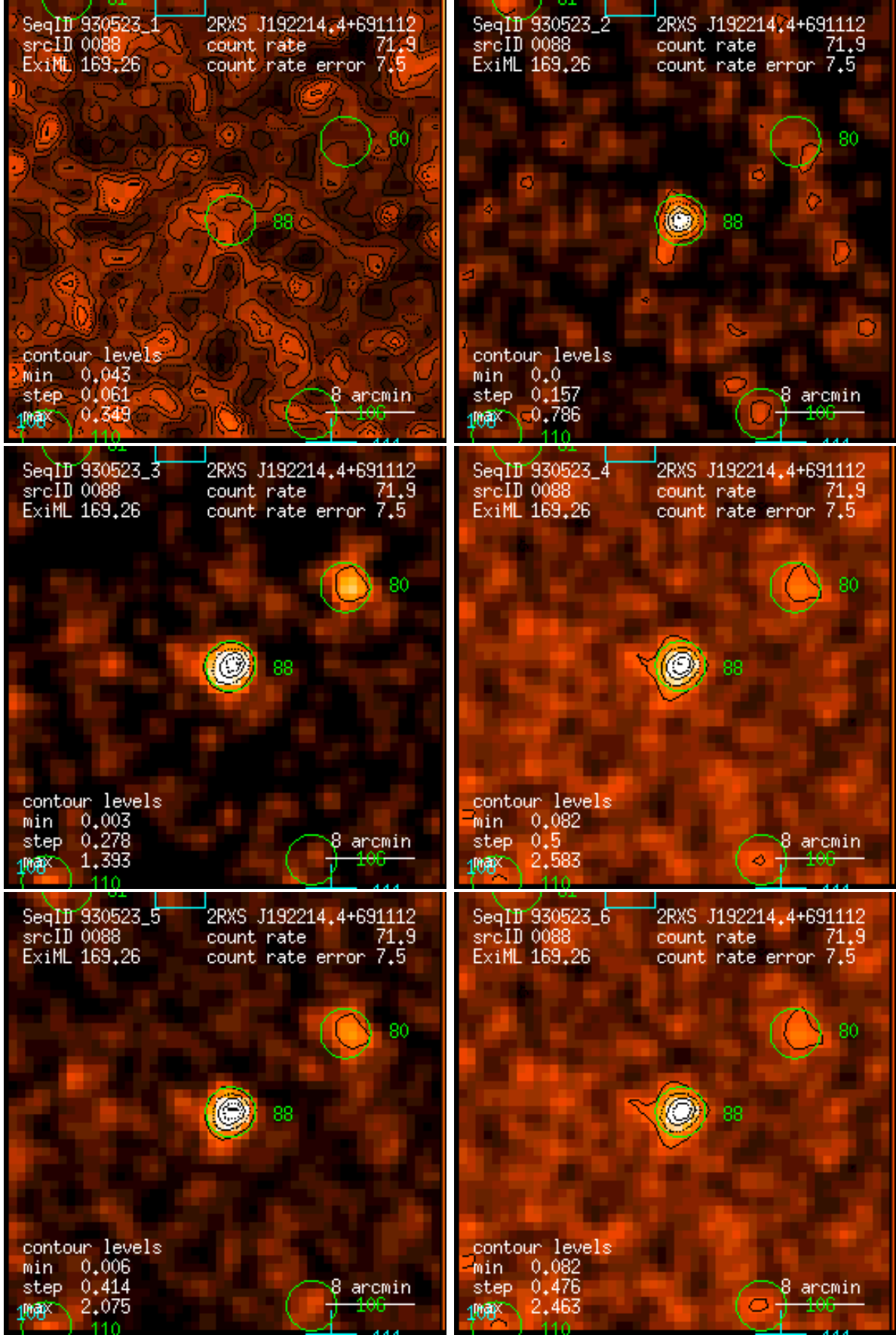
Figure 88: RASS 930523: detection 0088: band rate images, Gaussian filter: (1) PSPC channels 11 – 41, (2) 52 – 90, (3) 91 – 201, (4) 11 – 235, (5) 52 – 201, (6) 11 – 201. Broad band rates in counts/ks. Band rate contour levels in counts/ks/arcmin 2 .
