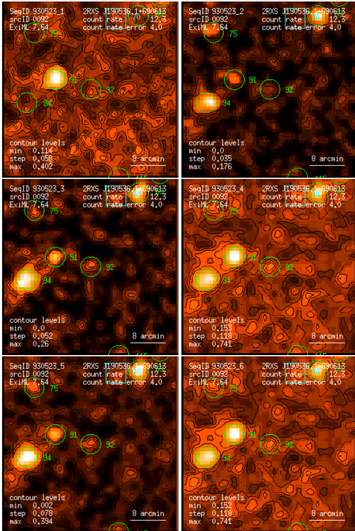
Figure 92: RASS 930523: detection 0092: band rate images, Gaussian filter: (1) PSPC channels 11 – 41, (2) 52 – 90, (3) 91 – 201, (4) 11 – 235, (5) 52 – 201, (6) 11 – 201. Broad band rates in counts/ks. Band rate contour levels in counts/ks/arcmin 2 .
