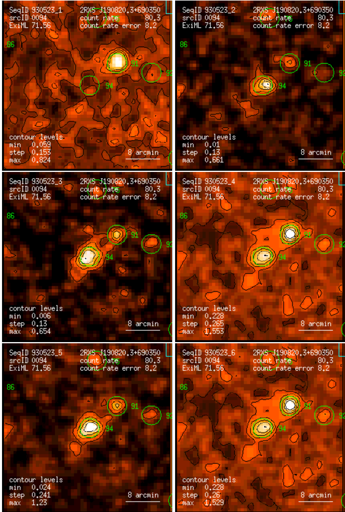
Figure 94: RASS 930523: detection 0094: band rate images, Gaussian filter: (1) PSPC channels 11 – 41, (2) 52 – 90, (3) 91 – 201, (4) 11 – 235, (5) 52 – 201, (6) 11 – 201. Broad band rates in counts/ks. Band rate contour levels in counts/ks/arcmin 2 .
