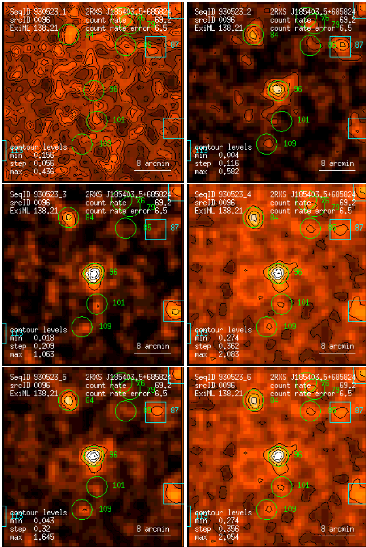
Figure 96: RASS 930523: detection 0096: band rate images, Gaussian filter: (1) PSPC channels 11 – 41, (2) 52 – 90, (3) 91 – 201, (4) 11 – 235, (5) 52 – 201, (6) 11 – 201. Broad band rates in counts/ks. Band rate contour levels in counts/ks/arcmin 2 .
