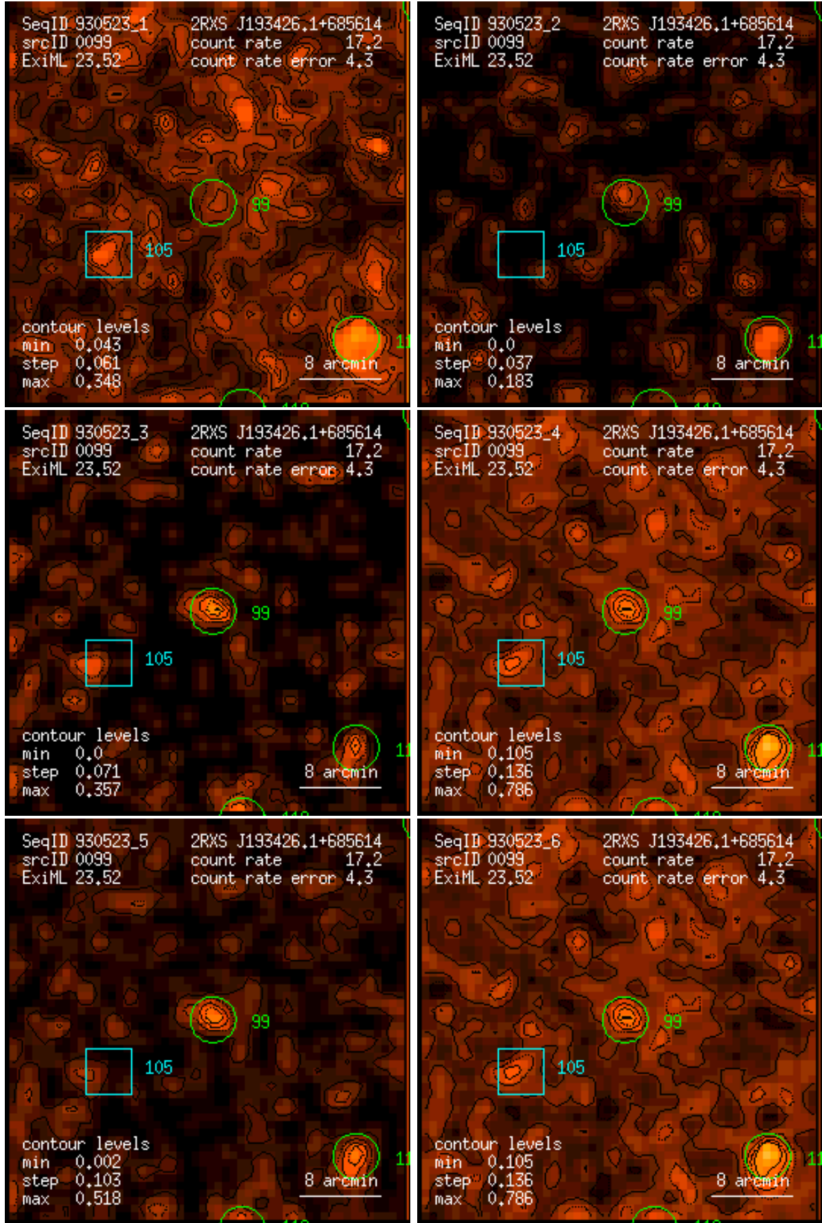
Figure 99: RASS 930523: detection 0099: band rate images, Gaussian filter: (1) PSPC channels 11 – 41, (2) 52 – 90, (3) 91 – 201, (4) 11 – 235, (5) 52 – 201, (6) 11 – 201. Broad band rates in counts/ks. Band rate contour levels in counts/ks/arcmin 2 .
