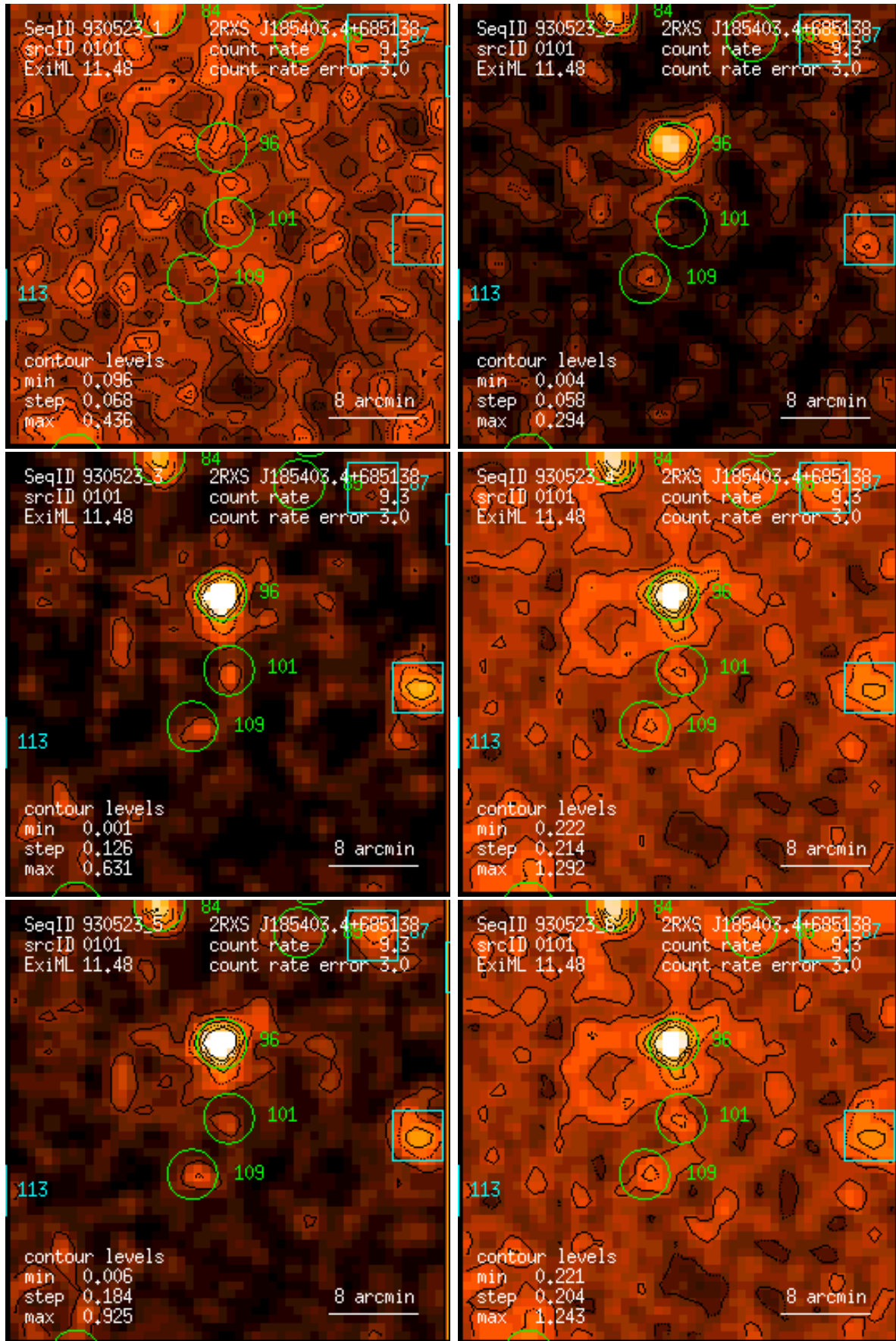
Figure 101: RASS 930523: detection 0101: band rate images, Gaussian filter: (1) PSPC channels 11 – 41, (2) 52 – 90, (3) 91 – 201, (4) 11 – 235, (5) 52 – 201, (6) 11 – 201. Broad band rates in counts/ks. Band rate contour levels in counts/ks/arcmin 2 .
