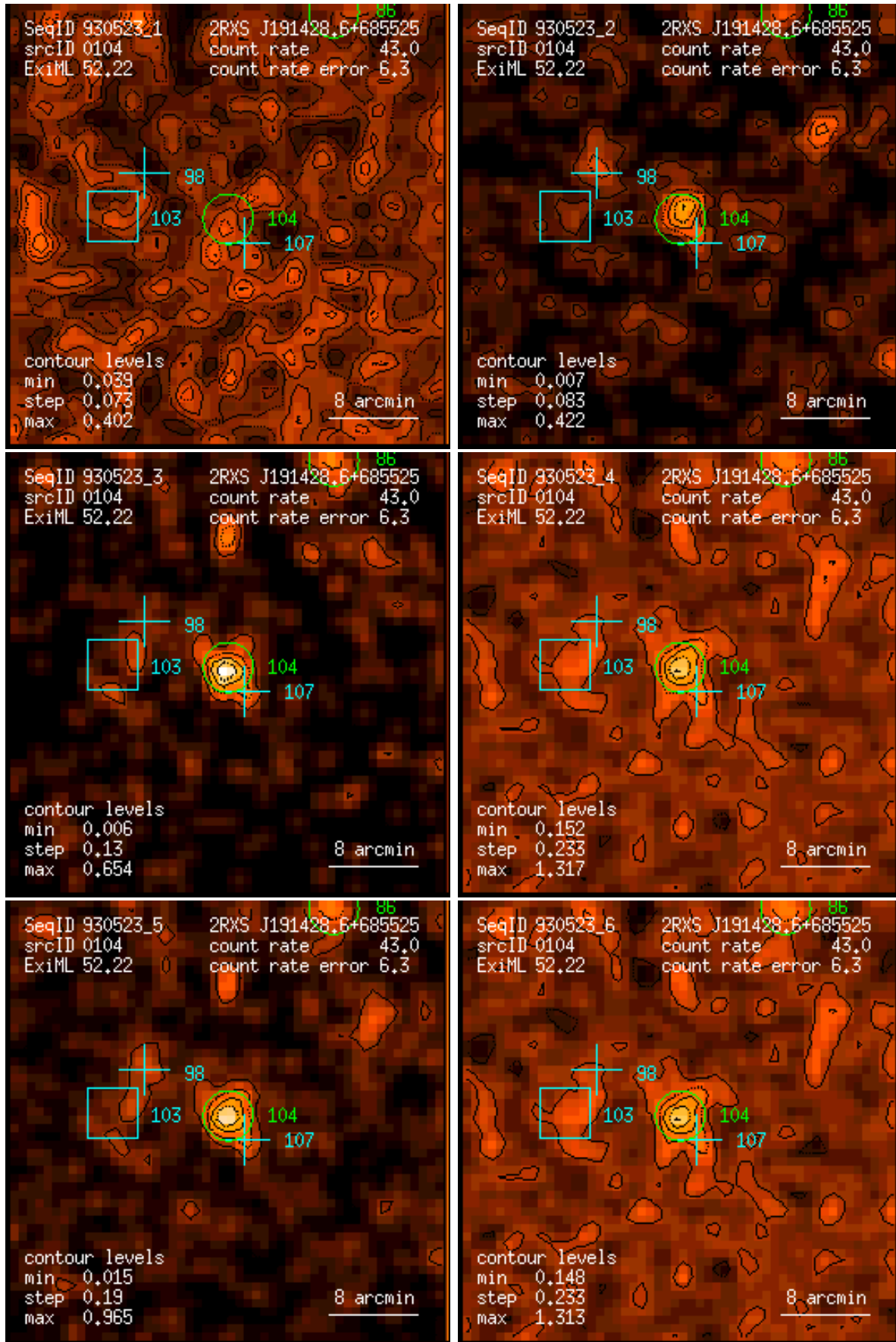
Figure 104: RASS 930523: detection 0104: band rate images, Gaussian filter: (1) PSPC channels 11 – 41, (2) 52 – 90, (3) 91 – 201, (4) 11 – 235, (5) 52 – 201, (6) 11 – 201. Broad band rates in counts/ks. Band rate contour levels in counts/ks/arcmin 2 .
