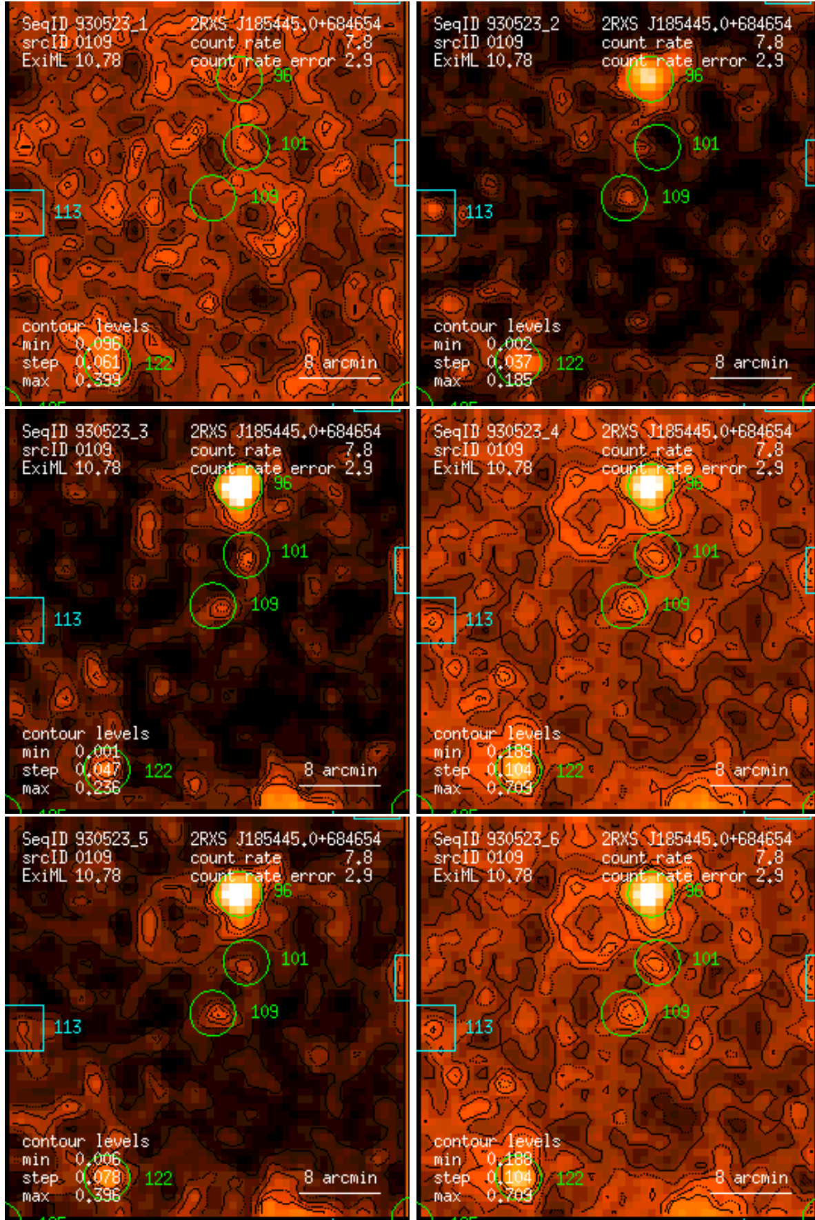
Figure 109: RASS 930523: detection 0109: band rate images, Gaussian filter: (1) PSPC channels 11 – 41, (2) 52 – 90, (3) 91 – 201, (4) 11 – 235, (5) 52 – 201, (6) 11 – 201. Broad band rates in counts/ks. Band rate contour levels in counts/ks/arcmin 2 .
