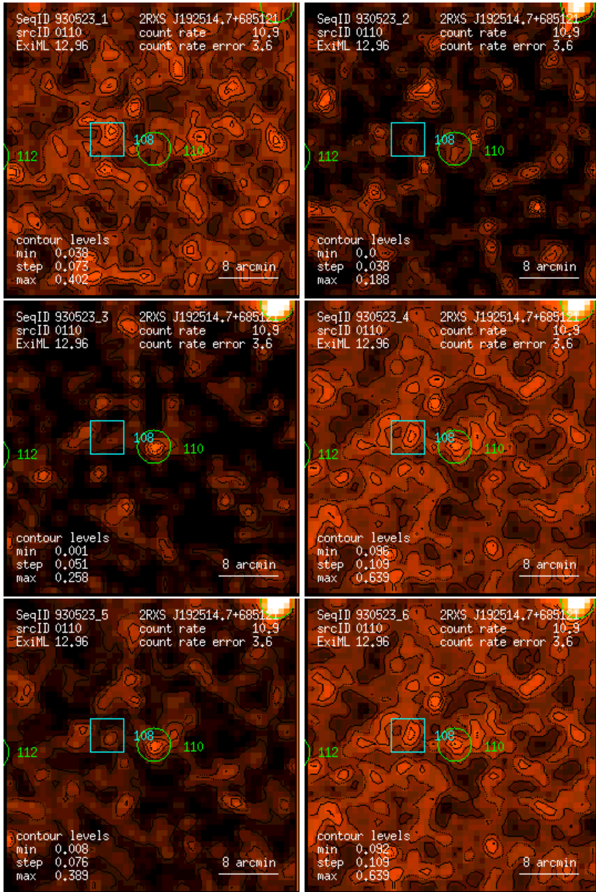
Figure 110: RASS 930523: detection 0110: band rate images, Gaussian filter: (1) PSPC channels 11 – 41, (2) 52 – 90, (3) 91 – 201, (4) 11 – 235, (5) 52 – 201, (6) 11 – 201. Broad band rates in counts/ks. Band rate contour levels in counts/ks/arcmin 2 .
