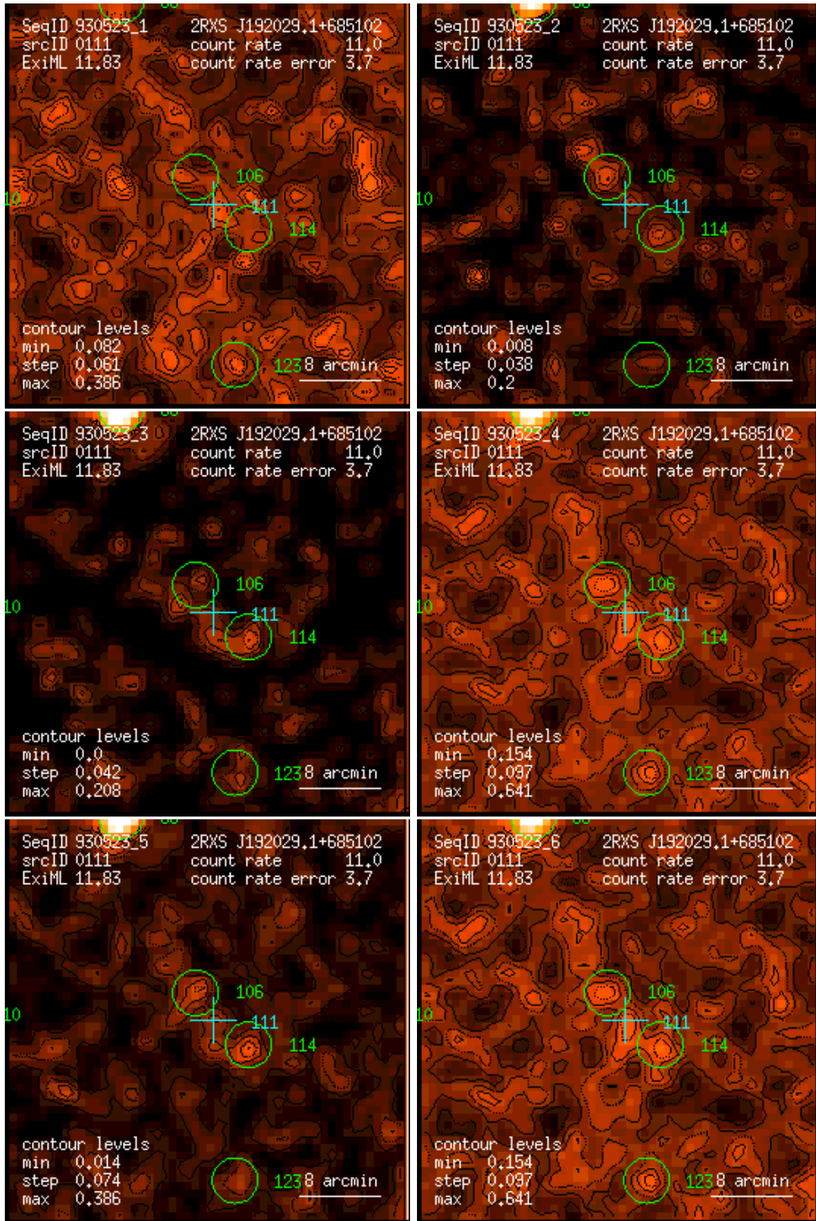
Figure 111: RASS 930523: detection 0111: band rate images, Gaussian filter: (1) PSPC channels 11 – 41, (2) 52 – 90, (3) 91 – 201, (4) 11 – 235, (5) 52 – 201, (6) 11 – 201. Broad band rates in counts/ks. Band rate contour levels in counts/ks/arcmin 2 .
