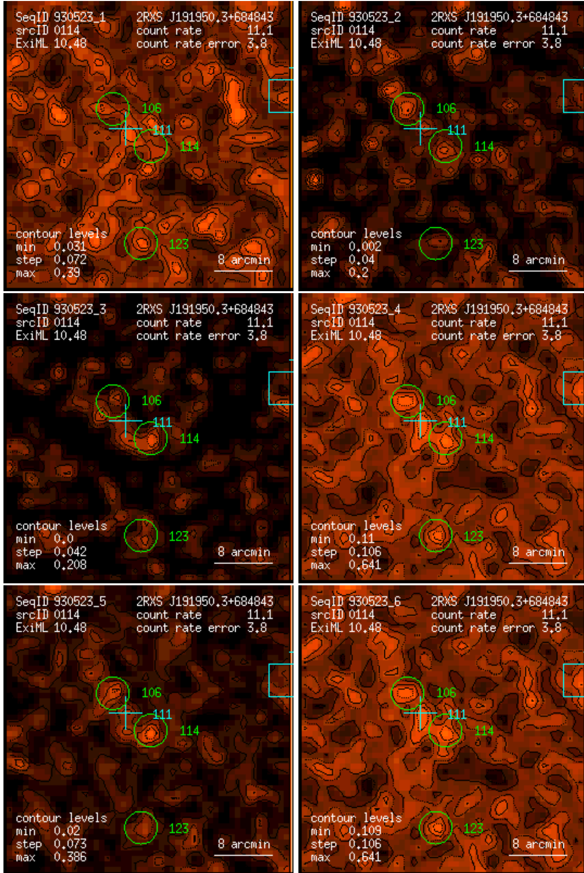
Figure 114: RASS 930523: detection 0114: band rate images, Gaussian filter: (1) PSPC channels 11 – 41, (2) 52 – 90, (3) 91 – 201, (4) 11 – 235, (5) 52 – 201, (6) 11 – 201. Broad band rates in counts/ks. Band rate contour levels in counts/ks/arcmin 2 .
