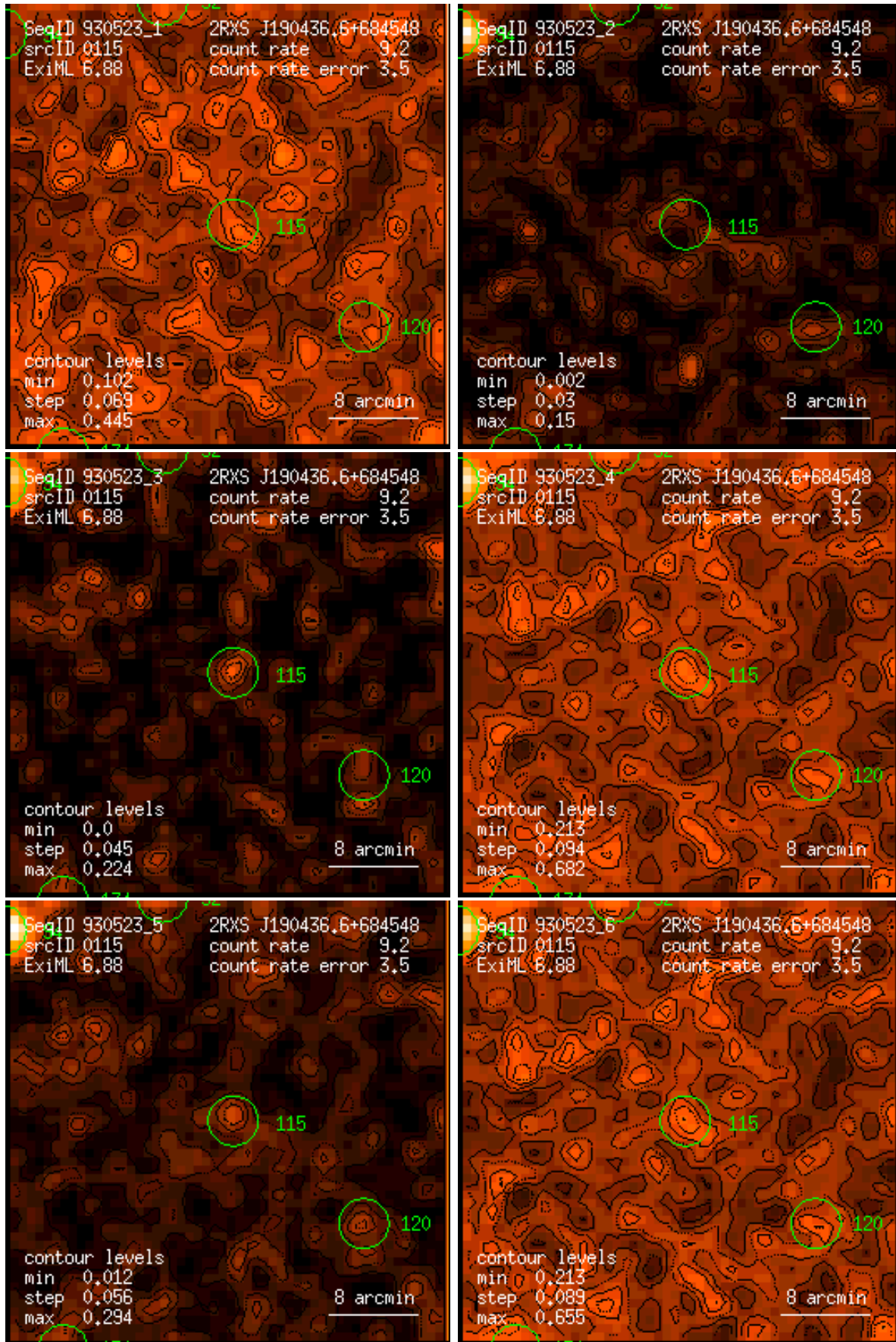
Figure 115: RASS 930523: detection 0115: band rate images, Gaussian filter: (1) PSPC channels 11 – 41, (2) 52 – 90, (3) 91 – 201, (4) 11 – 235, (5) 52 – 201, (6) 11 – 201. Broad band rates in counts/ks. Band rate contour levels in counts/ks/arcmin 2 .
