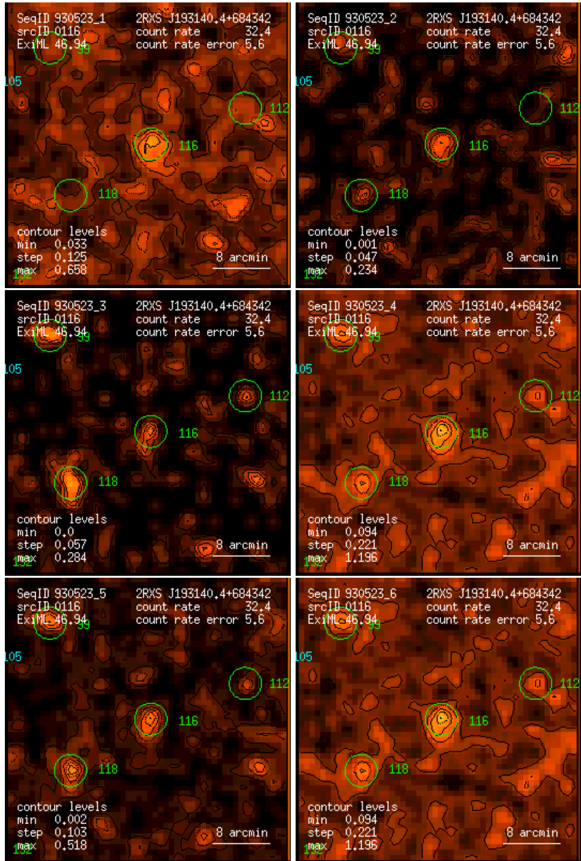
Figure 116: RASS 930523: detection 0116: band rate images, Gaussian filter: (1) PSPC channels 11 – 41, (2) 52 – 90, (3) 91 – 201, (4) 11 – 235, (5) 52 – 201, (6) 11 – 201. Broad band rates in counts/ks. Band rate contour levels in counts/ks/arcmin 2 .
