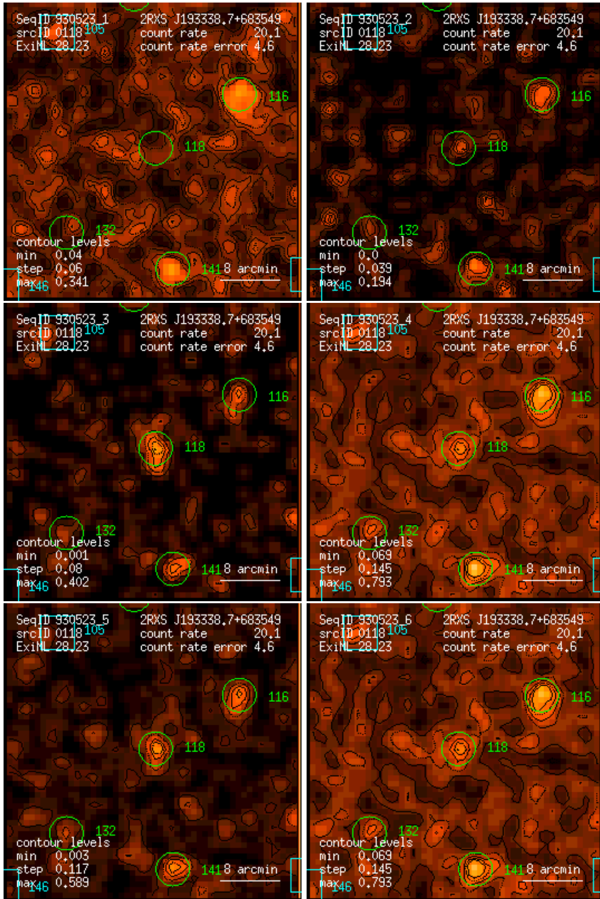
Figure 118: RASS 930523: detection 0118: band rate images, Gaussian filter: (1) PSPC channels 11 – 41, (2) 52 – 90, (3) 91 – 201, (4) 11 – 235, (5) 52 – 201, (6) 11 – 201. Broad band rates in counts/ks. Band rate contour levels in counts/ks/arcmin 2 .
