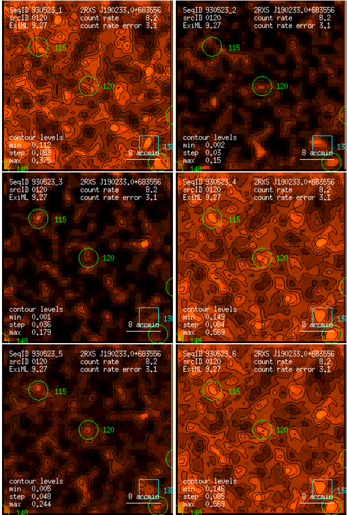
Figure 120: RASS 930523: detection 0120: band rate images, Gaussian filter: (1) PSPC channels 11 – 41, (2) 52 – 90, (3) 91 – 201, (4) 11 – 235, (5) 52 – 201, (6) 11 – 201. Broad band rates in counts/ks. Band rate contour levels in counts/ks/arcmin 2 .
