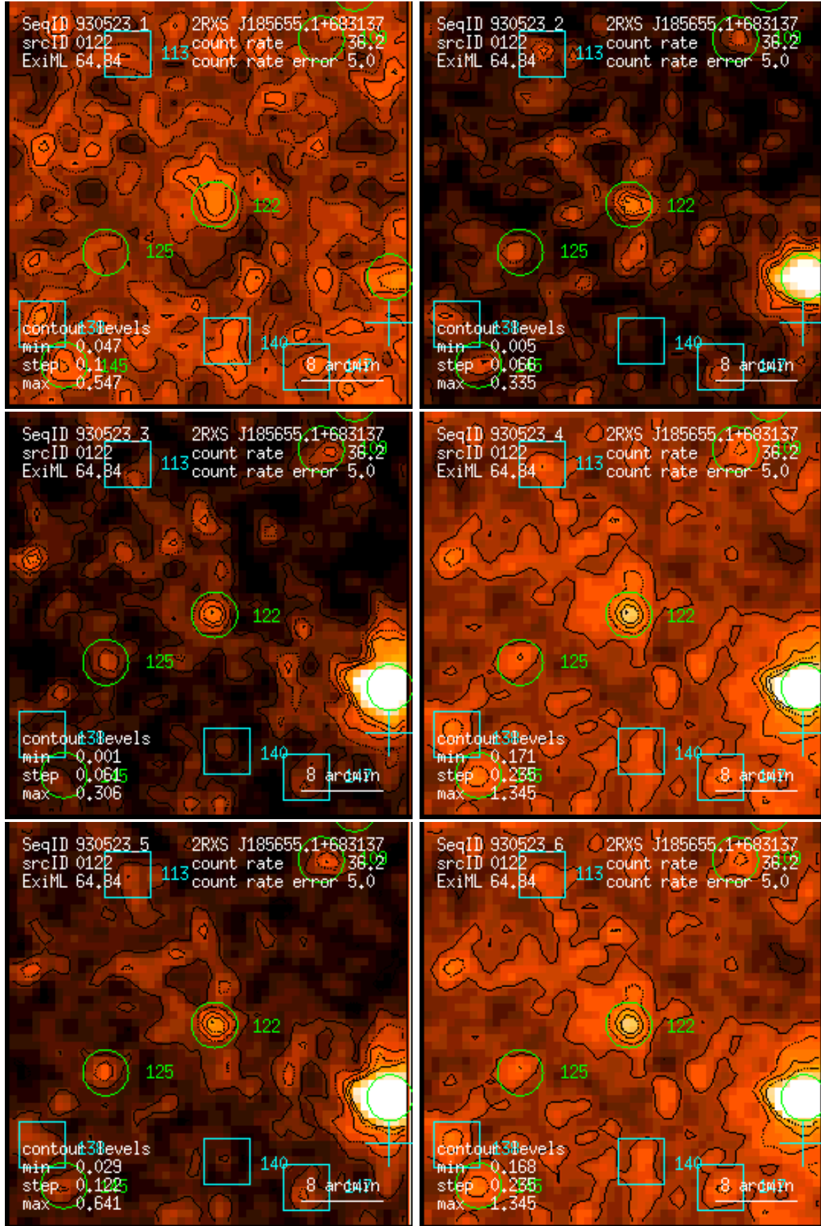
Figure 122: RASS 930523: detection 0122: band rate images, Gaussian filter: (1) PSPC channels 11 – 41, (2) 52 – 90, (3) 91 – 201, (4) 11 – 235, (5) 52 – 201, (6) 11 – 201. Broad band rates in counts/ks. Band rate contour levels in counts/ks/arcmin 2 .
