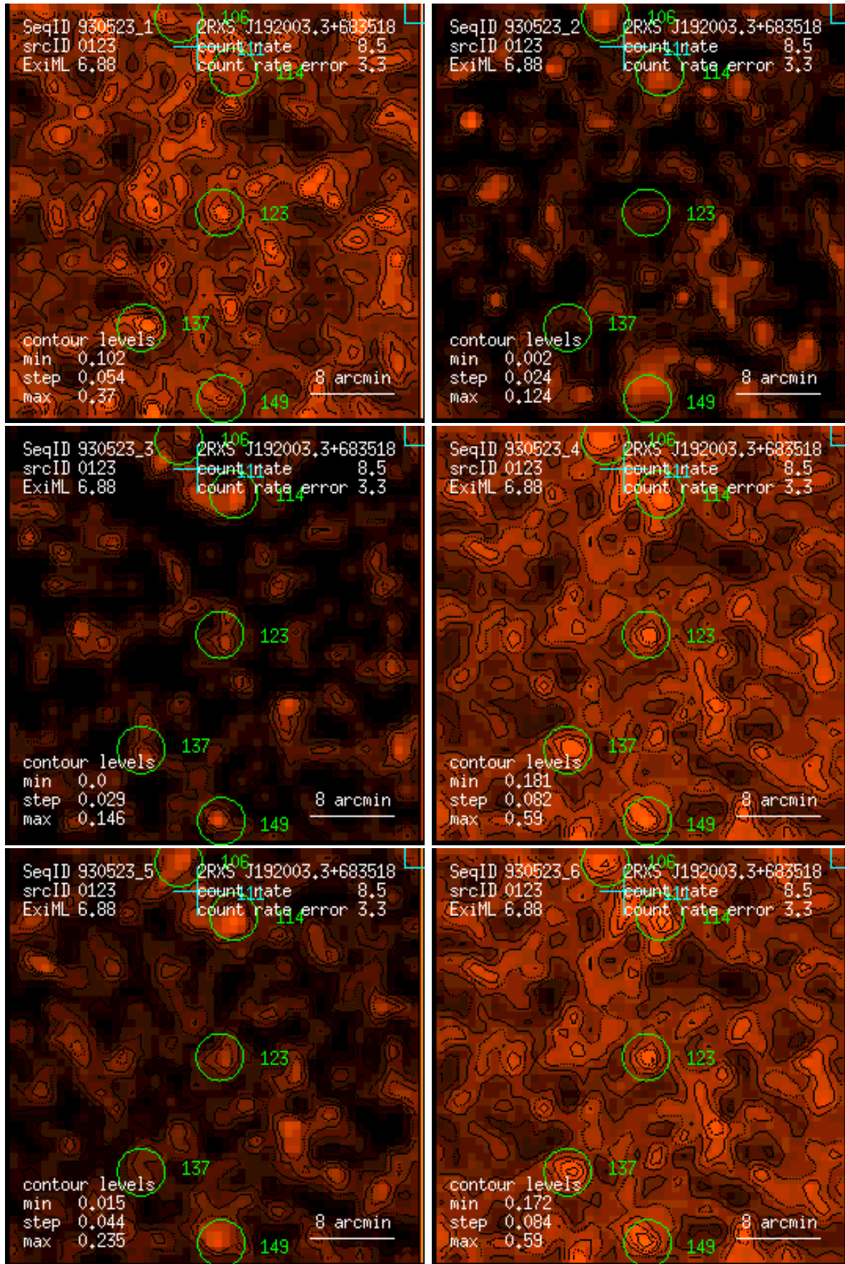
Figure 123: RASS 930523: detection 0123: band rate images, Gaussian filter: (1) PSPC channels 11 – 41, (2) 52 – 90, (3) 91 – 201, (4) 11 – 235, (5) 52 – 201, (6) 11 – 201. Broad band rates in counts/ks. Band rate contour levels in counts/ks/arcmin 2 .
