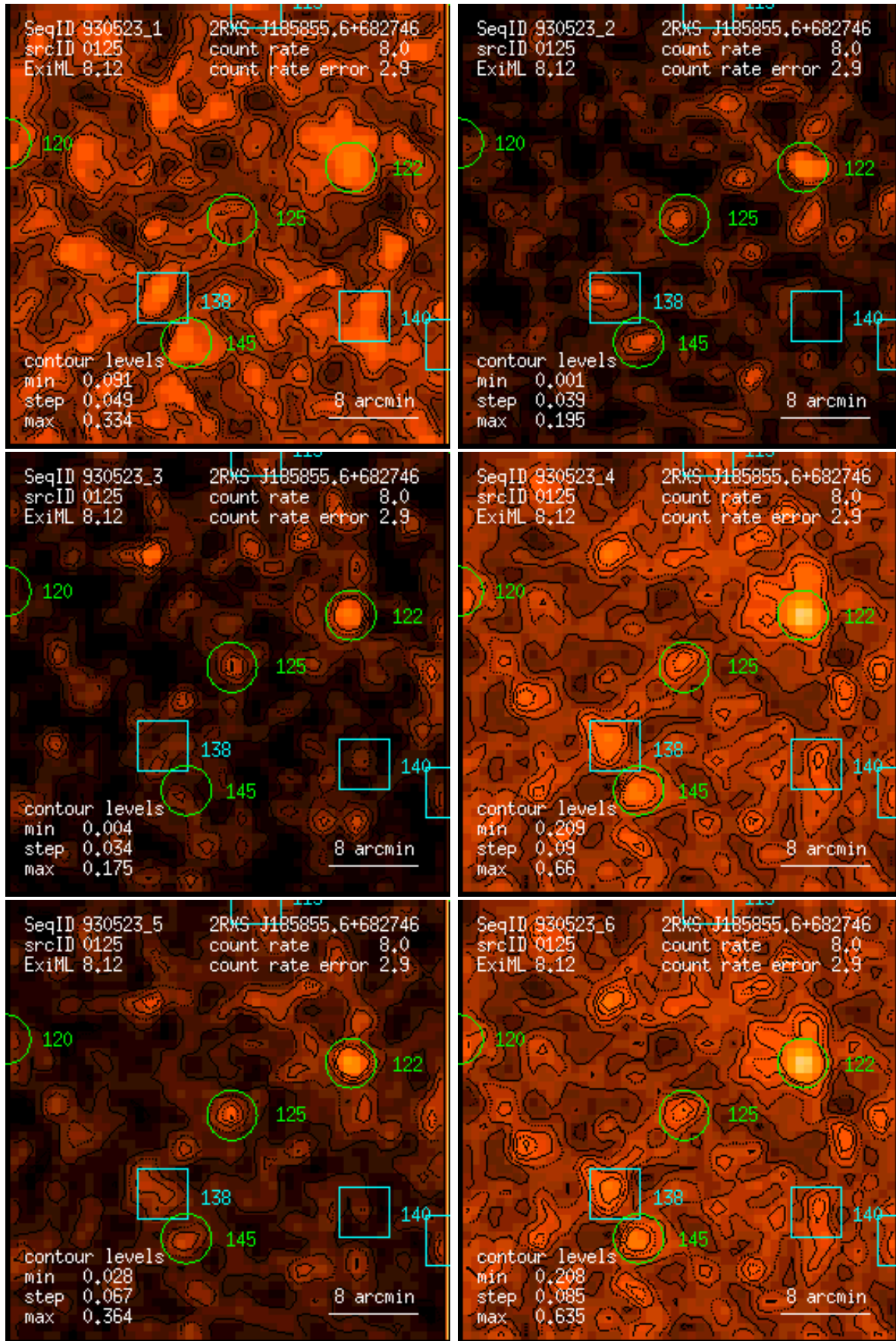
Figure 125: RASS 930523: detection 0125: band rate images, Gaussian filter: (1) PSPC channels 11 – 41, (2) 52 – 90, (3) 91 – 201, (4) 11 – 235, (5) 52 – 201, (6) 11 – 201. Broad band rates in counts/ks. Band rate contour levels in counts/ks/arcmin 2 .
