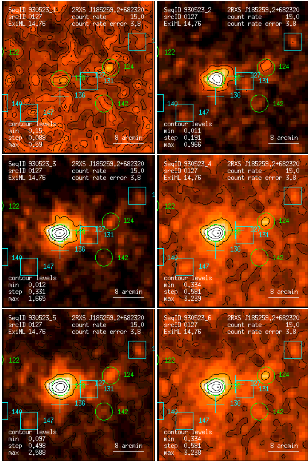
Figure 127: RASS 930523: detection 0127: band rate images, Gaussian filter: (1) PSPC channels 11 – 41, (2) 52 – 90, (3) 91 – 201, (4) 11 – 235, (5) 52 – 201, (6) 11 – 201. Broad band rates in counts/ks. Band rate contour levels in counts/ks/arcmin 2 .
