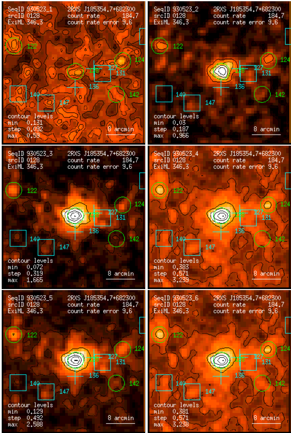
Figure 128: RASS 930523: detection 0128: band rate images, Gaussian filter: (1) PSPC channels 11 – 41, (2) 52 – 90, (3) 91 – 201, (4) 11 – 235, (5) 52 – 201, (6) 11 – 201. Broad band rates in counts/ks. Band rate contour levels in counts/ks/arcmin 2 .
