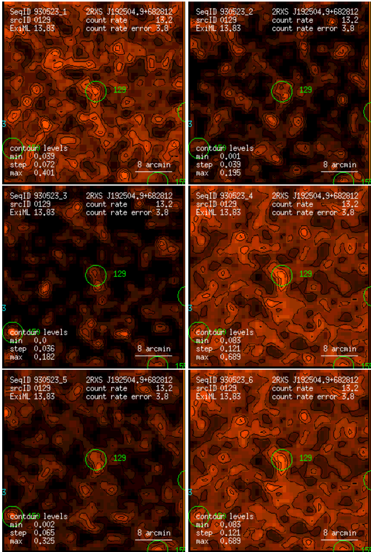
Figure 129: RASS 930523: detection 0129: band rate images, Gaussian filter: (1) PSPC channels 11 – 41, (2) 52 – 90, (3) 91 – 201, (4) 11 – 235, (5) 52 – 201, (6) 11 – 201. Broad band rates in counts/ks. Band rate contour levels in counts/ks/arcmin 2 .
