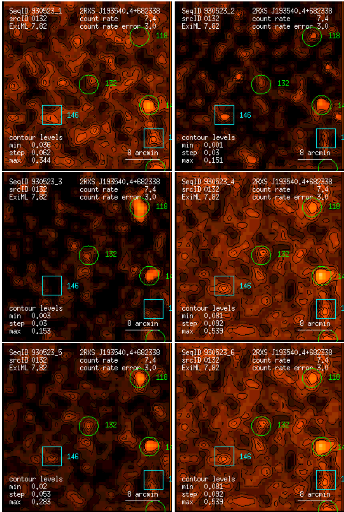
Figure 132: RASS 930523: detection 0132: band rate images, Gaussian filter: (1) PSPC channels 11 – 41, (2) 52 – 90, (3) 91 – 201, (4) 11 – 235, (5) 52 – 201, (6) 11 – 201. Broad band rates in counts/ks. Band rate contour levels in counts/ks/arcmin 2 .
