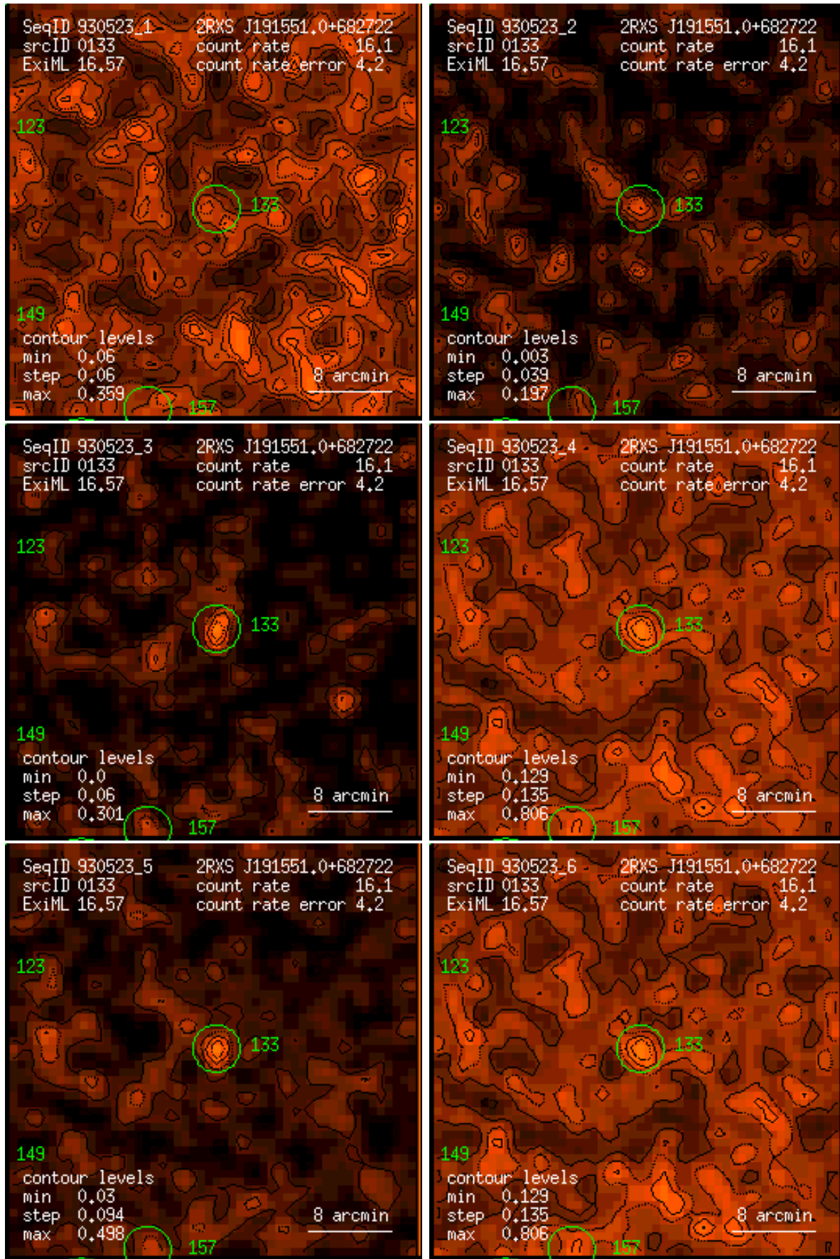
Figure 133: RASS 930523: detection 0133: band rate images, Gaussian filter: (1) PSPC channels 11 – 41, (2) 52 – 90, (3) 91 – 201, (4) 11 – 235, (5) 52 – 201, (6) 11 – 201. Broad band rates in counts/ks. Band rate contour levels in counts/ks/arcmin 2 .
