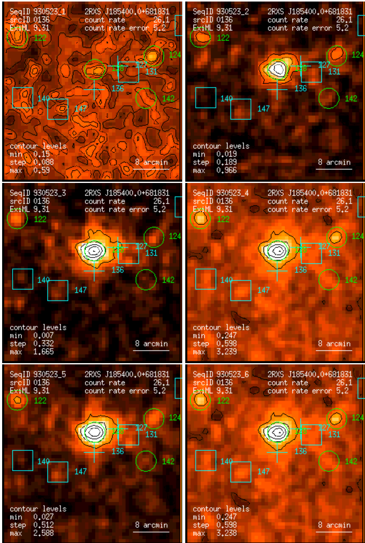
Figure 136: RASS 930523: detection 0136: band rate images, Gaussian filter: (1) PSPC channels 11 – 41, (2) 52 – 90, (3) 91 – 201, (4) 11 – 235, (5) 52 – 201, (6) 11 – 201. Broad band rates in counts/ks. Band rate contour levels in counts/ks/arcmin 2 .
