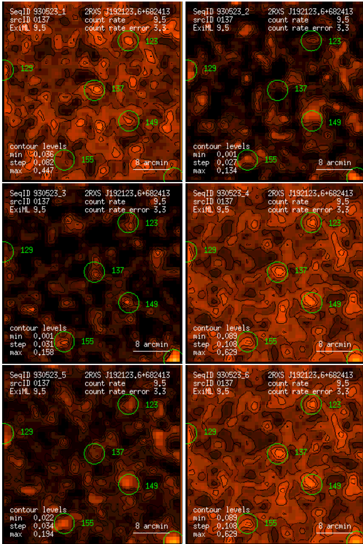
Figure 137: RASS 930523: detection 0137: band rate images, Gaussian filter: (1) PSPC channels 11 – 41, (2) 52 – 90, (3) 91 – 201, (4) 11 – 235, (5) 52 – 201, (6) 11 – 201. Broad band rates in counts/ks. Band rate contour levels in counts/ks/arcmin 2 .
