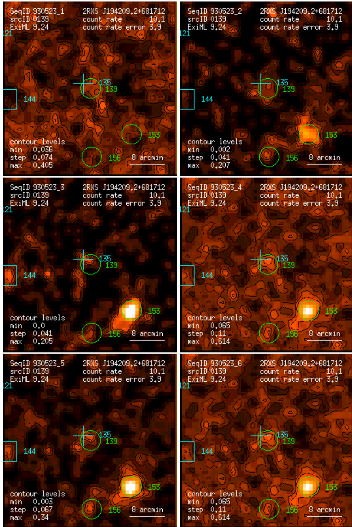
Figure 139: RASS 930523: detection 0139: band rate images, Gaussian filter: (1) PSPC channels 11 – 41, (2) 52 – 90, (3) 91 – 201, (4) 11 – 235, (5) 52 – 201, (6) 11 – 201. Broad band rates in counts/ks. Band rate contour levels in counts/ks/arcmin 2 .
