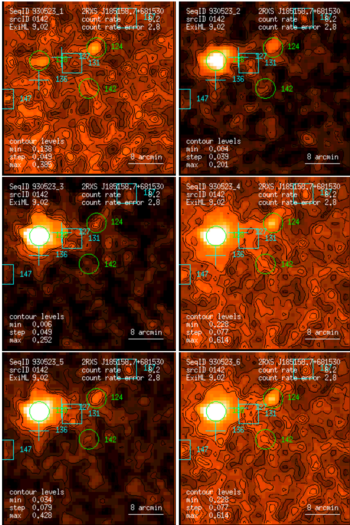
Figure 142: RASS 930523: detection 0142: band rate images, Gaussian filter: (1) PSPC channels 11 – 41, (2) 52 – 90, (3) 91 – 201, (4) 11 – 235, (5) 52 – 201, (6) 11 – 201. Broad band rates in counts/ks. Band rate contour levels in counts/ks/arcmin 2 .
