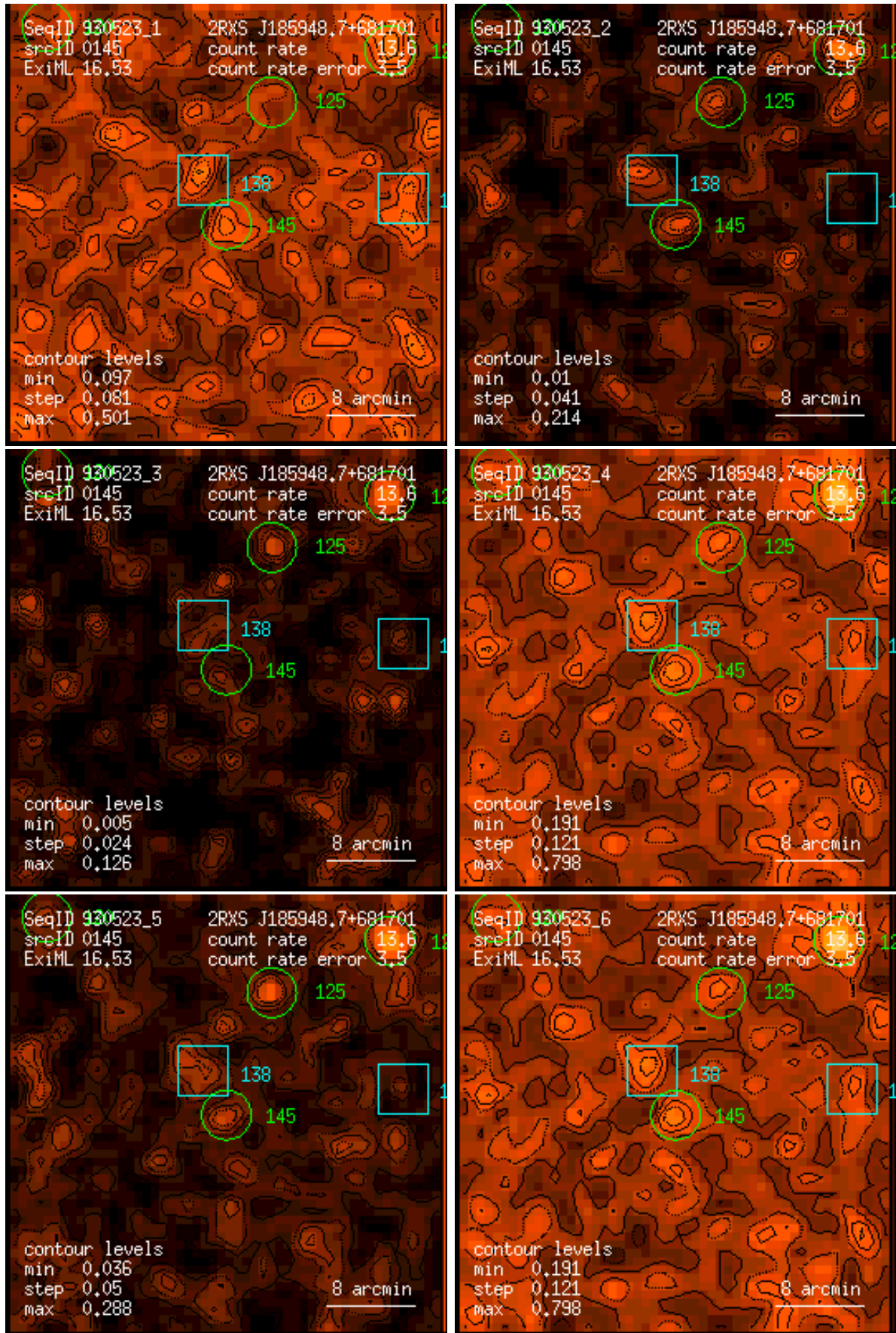
Figure 145: RASS 930523: detection 0145: band rate images, Gaussian filter: (1) PSPC channels 11 – 41, (2) 52 – 90, (3) 91 – 201, (4) 11 – 235, (5) 52 – 201, (6) 11 – 201. Broad band rates in counts/ks. Band rate contour levels in counts/ks/arcmin 2 .
