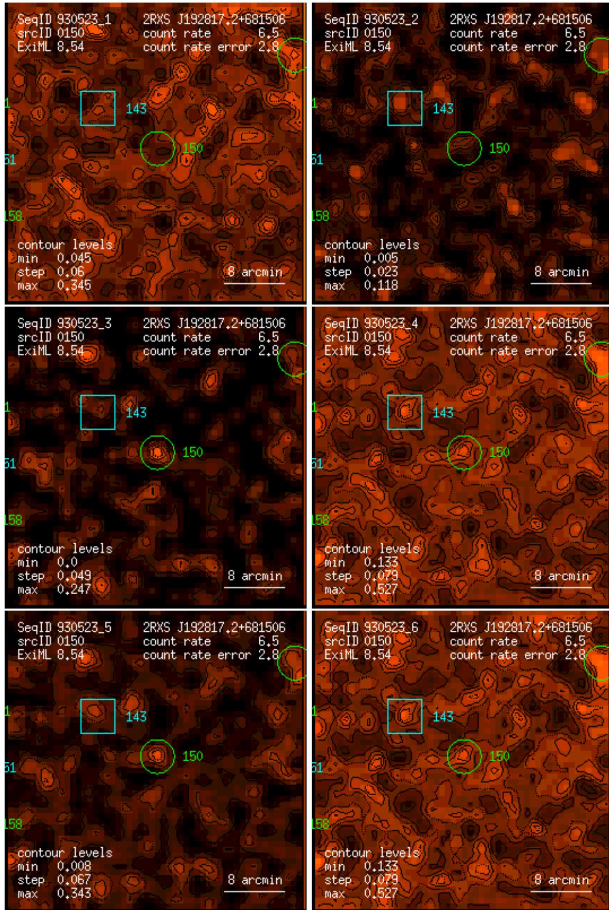
Figure 150: RASS 930523: detection 0150: band rate images, Gaussian filter: (1) PSPC channels 11 – 41, (2) 52 – 90, (3) 91 – 201, (4) 11 – 235, (5) 52 – 201, (6) 11 – 201. Broad band rates in counts/ks. Band rate contour levels in counts/ks/arcmin 2 .
