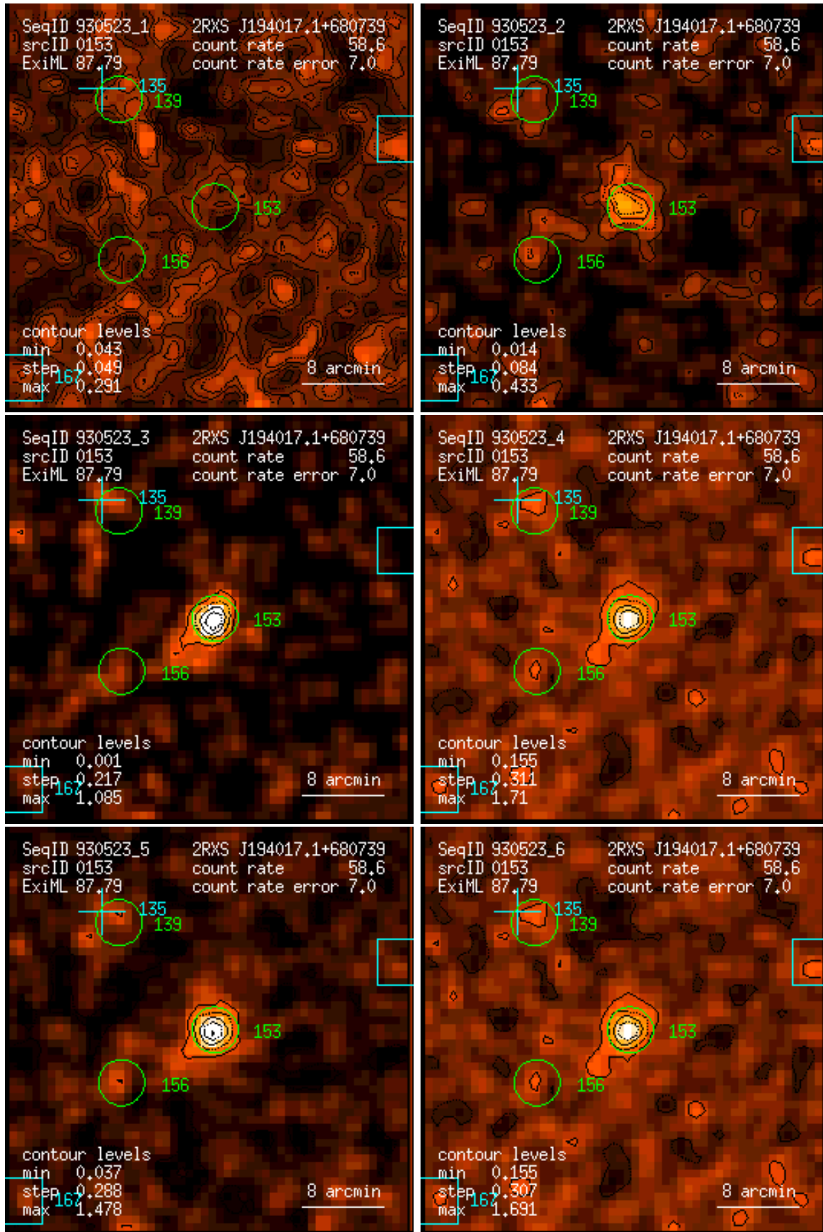
Figure 153: RASS 930523: detection 0153: band rate images, Gaussian filter: (1) PSPC channels 11 – 41, (2) 52 – 90, (3) 91 – 201, (4) 11 – 235, (5) 52 – 201, (6) 11 – 201. Broad band rates in counts/ks. Band rate contour levels in counts/ks/arcmin 2 .
