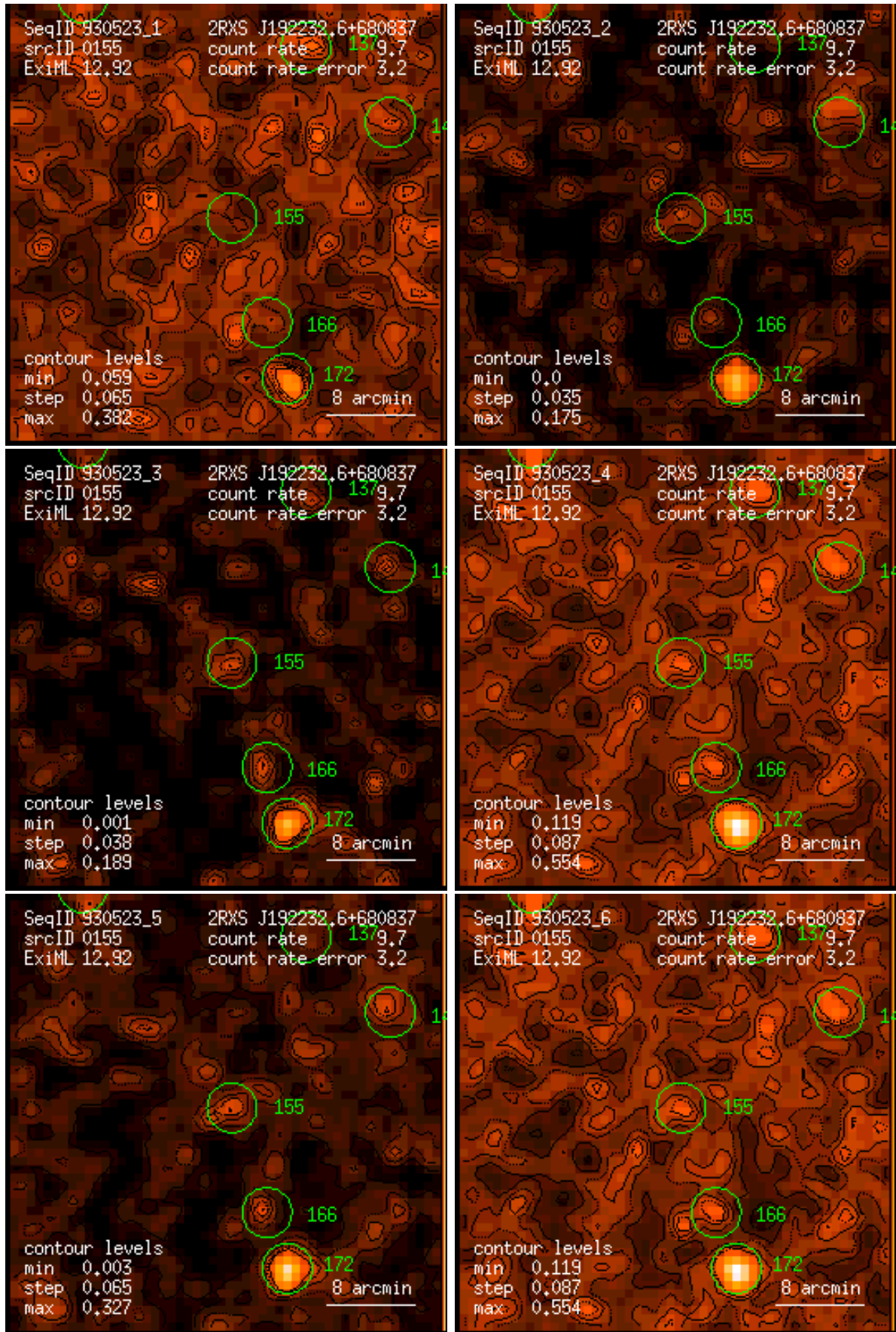
Figure 155: RASS 930523: detection 0155: band rate images, Gaussian filter: (1) PSPC channels 11 – 41, (2) 52 – 90, (3) 91 – 201, (4) 11 – 235, (5) 52 – 201, (6) 11 – 201. Broad band rates in counts/ks. Band rate contour levels in counts/ks/arcmin 2 .
