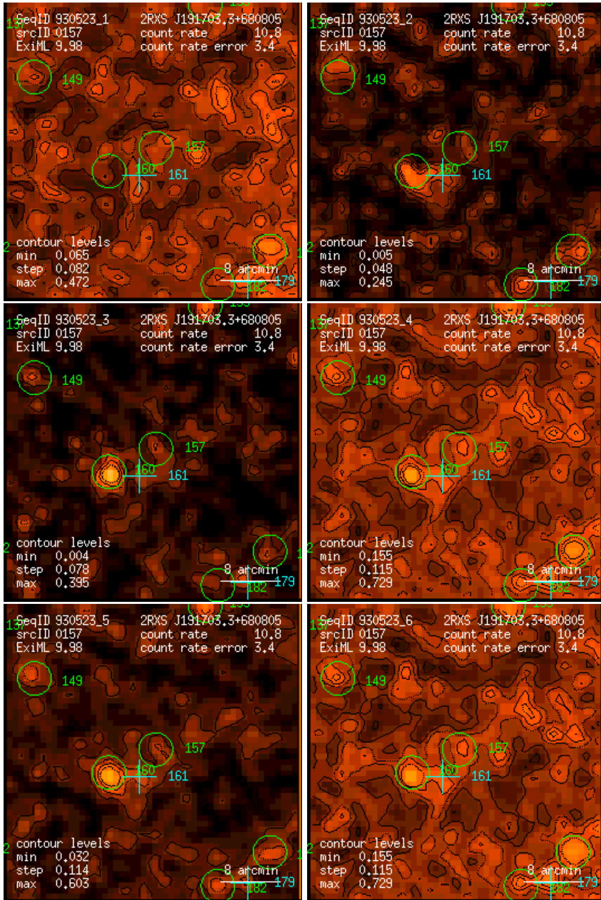
Figure 157: RASS 930523: detection 0157: band rate images, Gaussian filter: (1) PSPC channels 11 – 41, (2) 52 – 90, (3) 91 – 201, (4) 11 – 235, (5) 52 – 201, (6) 11 – 201. Broad band rates in counts/ks. Band rate contour levels in counts/ks/arcmin 2 .
