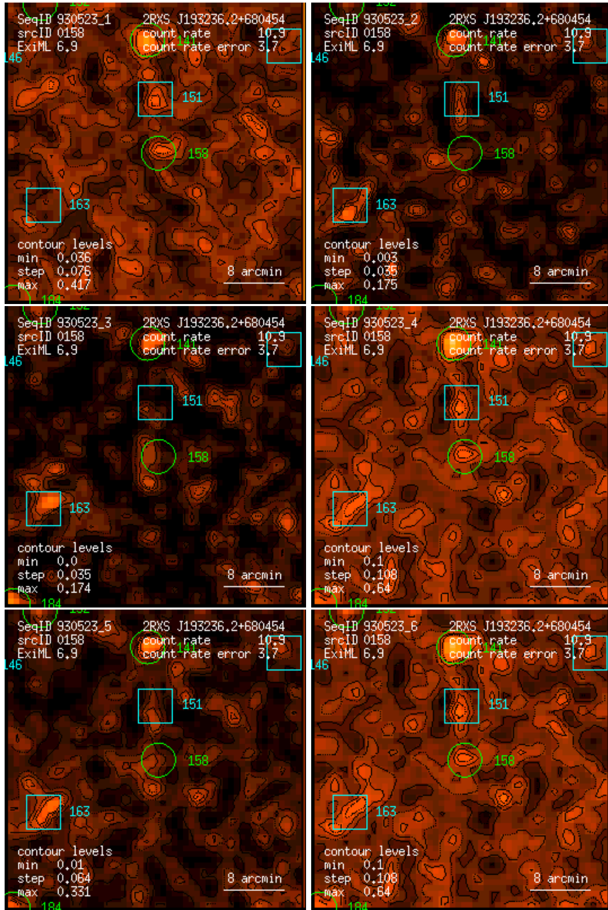
Figure 158: RASS 930523: detection 0158: band rate images, Gaussian filter: (1) PSPC channels 11 – 41, (2) 52 – 90, (3) 91 – 201, (4) 11 – 235, (5) 52 – 201, (6) 11 – 201. Broad band rates in counts/ks. Band rate contour levels in counts/ks/arcmin 2 .
