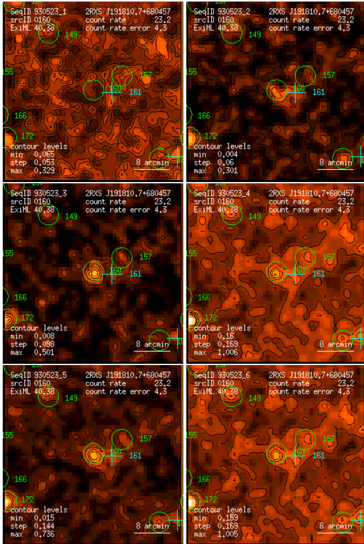
Figure 160: RASS 930523: detection 0160: band rate images, Gaussian filter: (1) PSPC channels 11 – 41, (2) 52 – 90, (3) 91 – 201, (4) 11 – 235, (5) 52 – 201, (6) 11 – 201. Broad band rates in counts/ks. Band rate contour levels in counts/ks/arcmin 2 .
