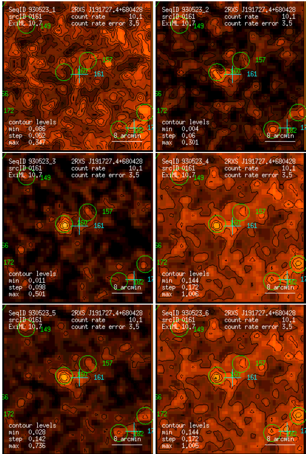
Figure 161: RASS 930523: detection 0161: band rate images, Gaussian filter: (1) PSPC channels 11 – 41, (2) 52 – 90, (3) 91 – 201, (4) 11 – 235, (5) 52 – 201, (6) 11 – 201. Broad band rates in counts/ks. Band rate contour levels in counts/ks/arcmin 2 .
