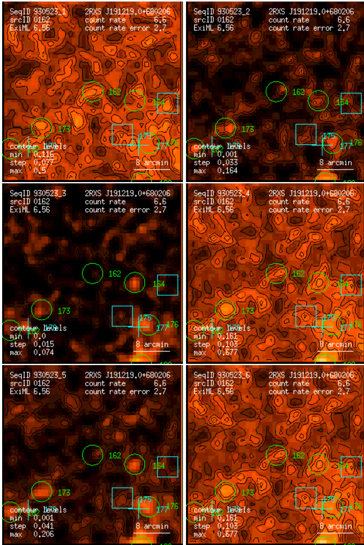
Figure 162: RASS 930523: detection 0162: band rate images, Gaussian filter: (1) PSPC channels 11 – 41, (2) 52 – 90, (3) 91 – 201, (4) 11 – 235, (5) 52 – 201, (6) 11 – 201. Broad band rates in counts/ks. Band rate contour levels in counts/ks/arcmin 2 .
