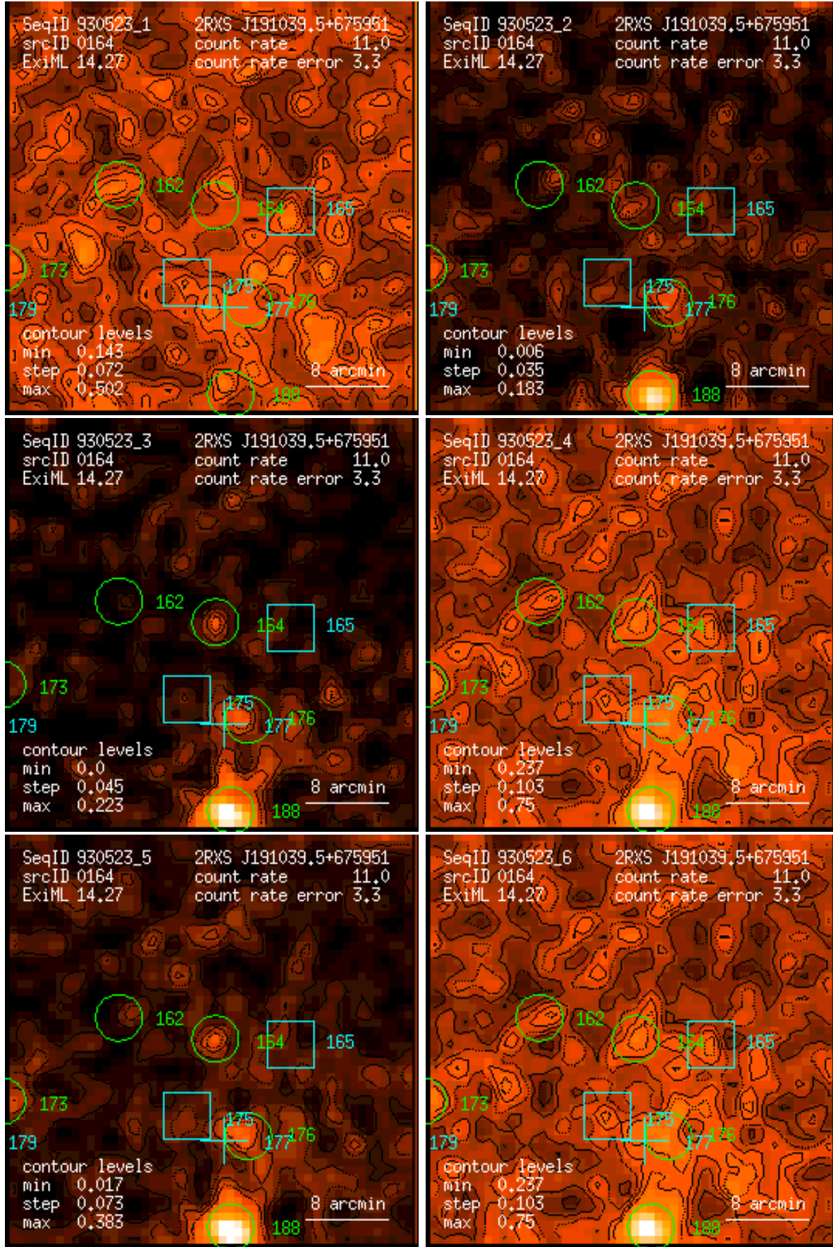
Figure 164: RASS 930523: detection 0164: band rate images, Gaussian filter: (1) PSPC channels 11 – 41, (2) 52 – 90, (3) 91 – 201, (4) 11 – 235, (5) 52 – 201, (6) 11 – 201. Broad band rates in counts/ks. Band rate contour levels in counts/ks/arcmin 2 .
