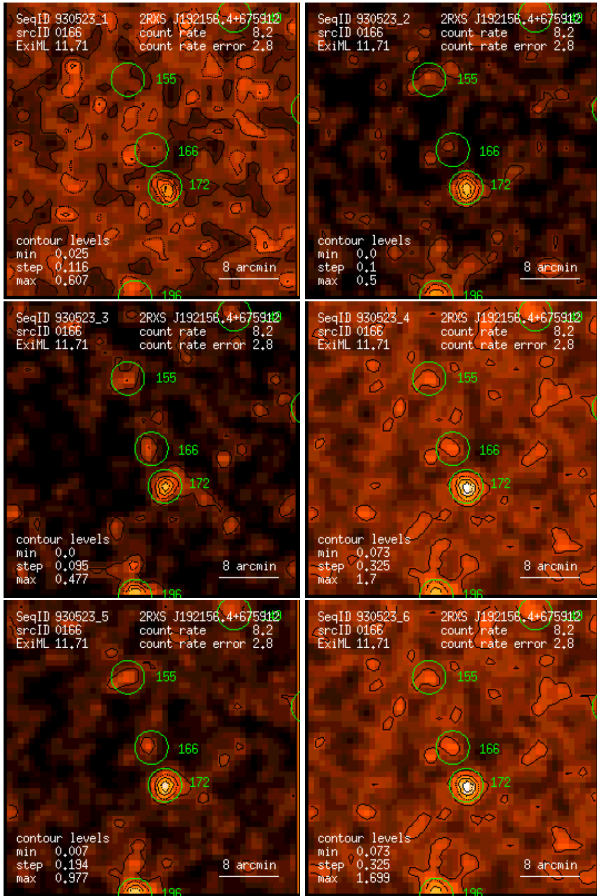
Figure 166: RASS 930523: detection 0166: band rate images, Gaussian filter: (1) PSPC channels 11 – 41, (2) 52 – 90, (3) 91 – 201, (4) 11 – 235, (5) 52 – 201, (6) 11 – 201. Broad band rates in counts/ks. Band rate contour levels in counts/ks/arcmin 2 .
