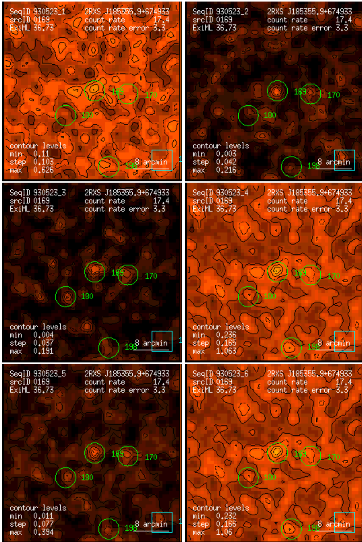
Figure 169: RASS 930523: detection 0169: band rate images, Gaussian filter: (1) PSPC channels 11 – 41, (2) 52 – 90, (3) 91 – 201, (4) 11 – 235, (5) 52 – 201, (6) 11 – 201. Broad band rates in counts/ks. Band rate contour levels in counts/ks/arcmin 2 .
